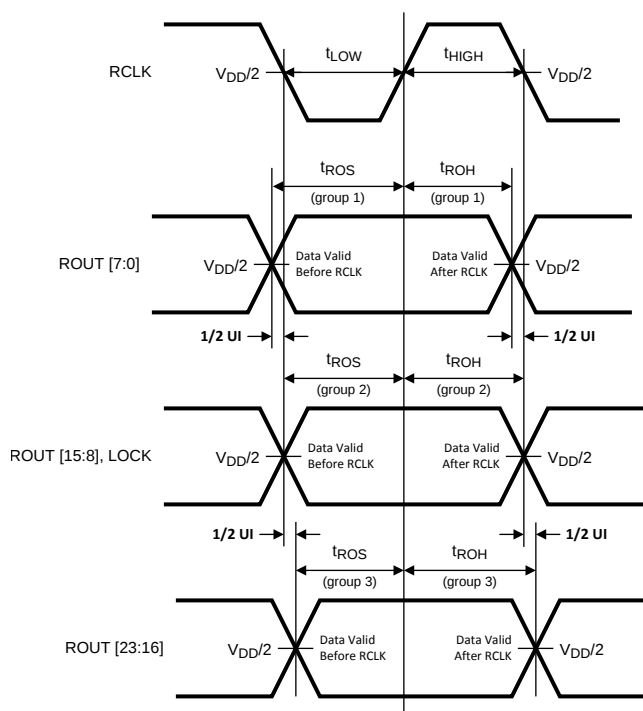
Figure 17. Deserializer Setup and Hold Times
