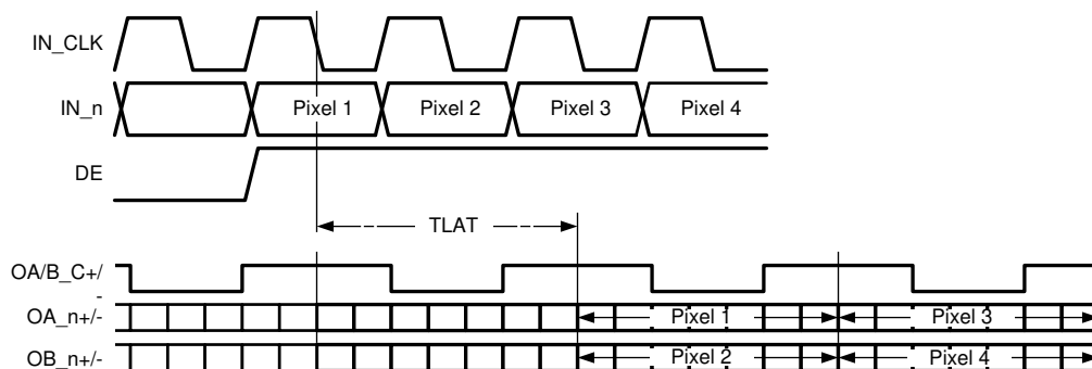
Figure 7-10. Single In, Dual Out Mode Timing and Latency
