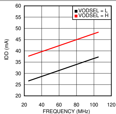
Figure 7-13. Typical Current Draw — Single In/Single Out Mode — PRBS-7 Data Pattern
