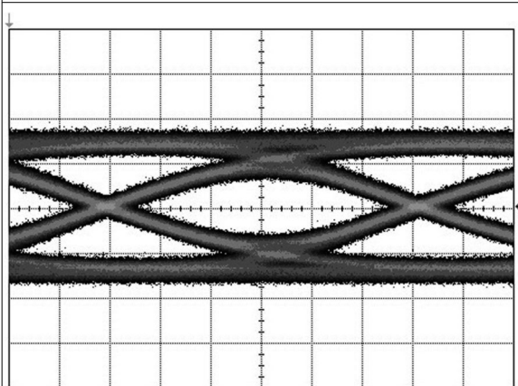
A. DS80PCI402 Settings: EQ[1:0] = [R, R] or 0x15, DEM[1:0] = [Float, Float]
