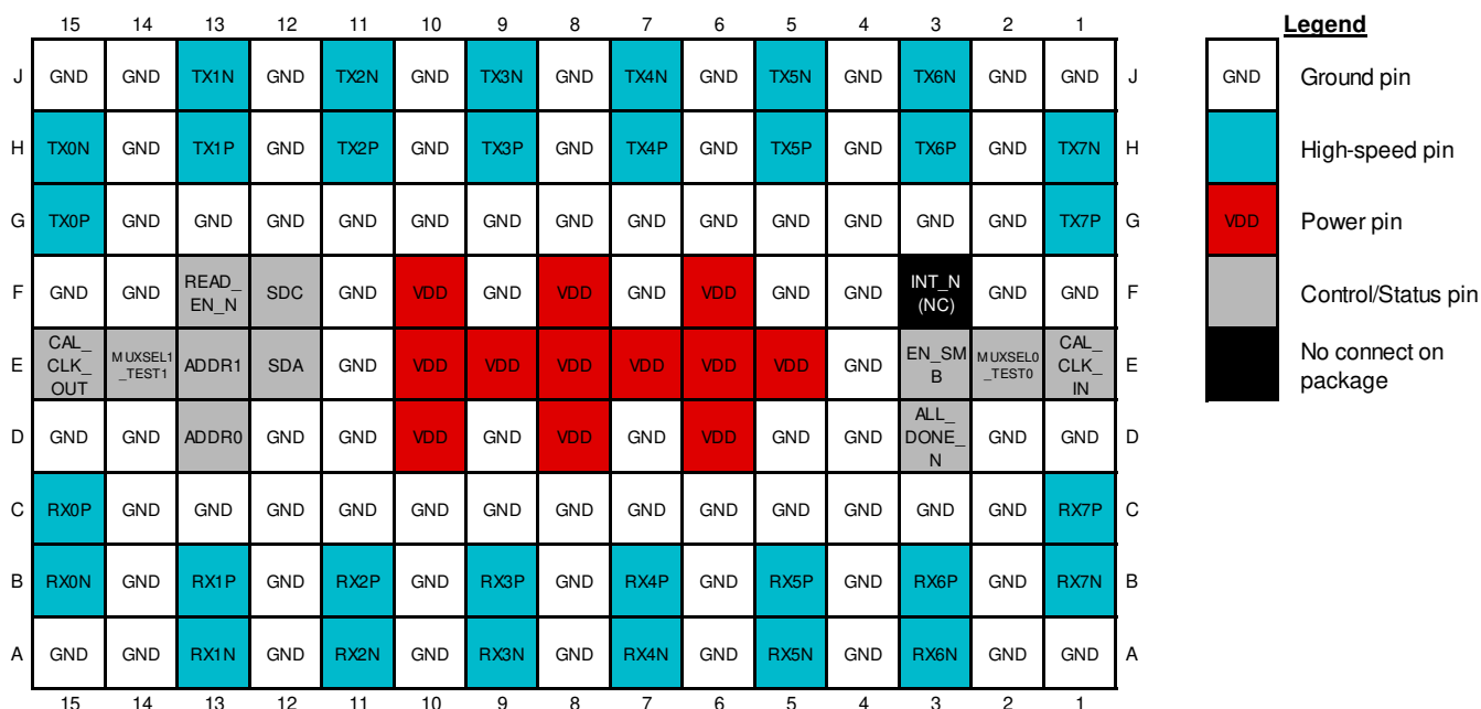
Figure 6-1. Top View
