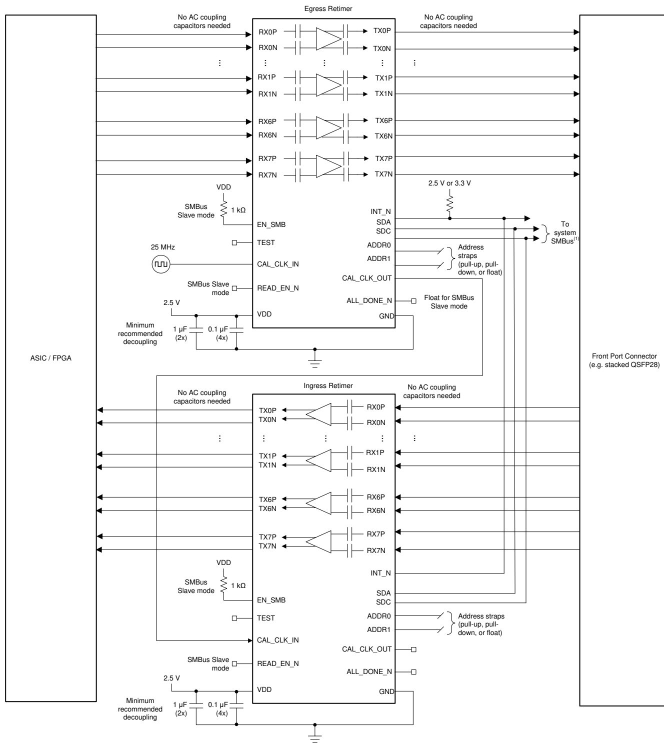
Figure 7-5. Front-Port Application Schematic
