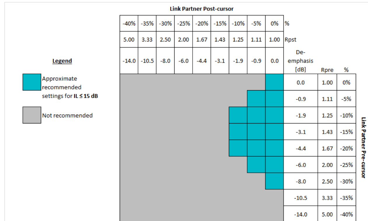
Figure 6-7. Guideline for Link partner FIR Settings When IL ≤ 15dB
