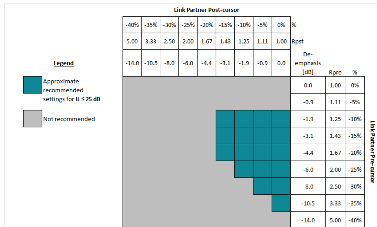
Figure 6-8. Guideline for Link partner FIR Settings When IL ≤ 25dB
