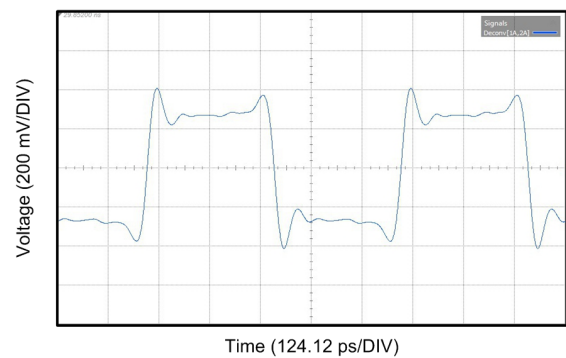
Figure 19. DS250DF410 FIR Transmit Equalization While Operating at 25.78125 Gbps
