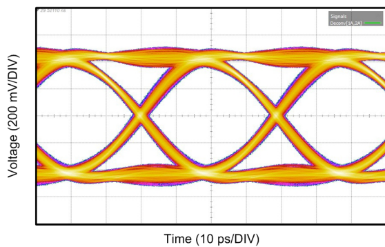
Figure 18. DS250DF410 Operating at 25.78125 Gbps
