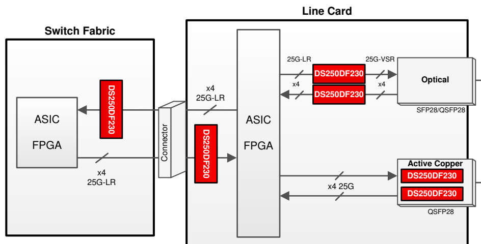
Figure 9-1. Typical Uses for the DS250DF230 in a System
