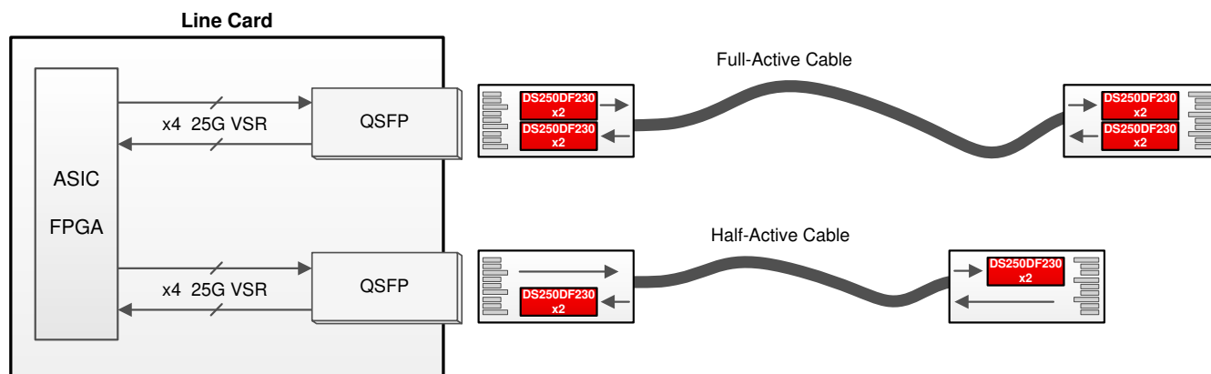
Figure 9-7. Active Cable Application Block Diagram
