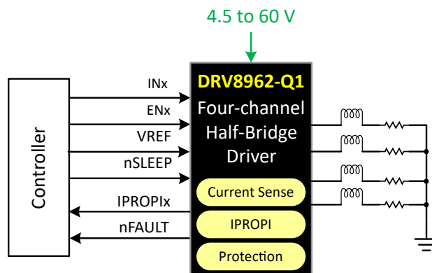
DRV8962-Q1 Simplified Schematic
