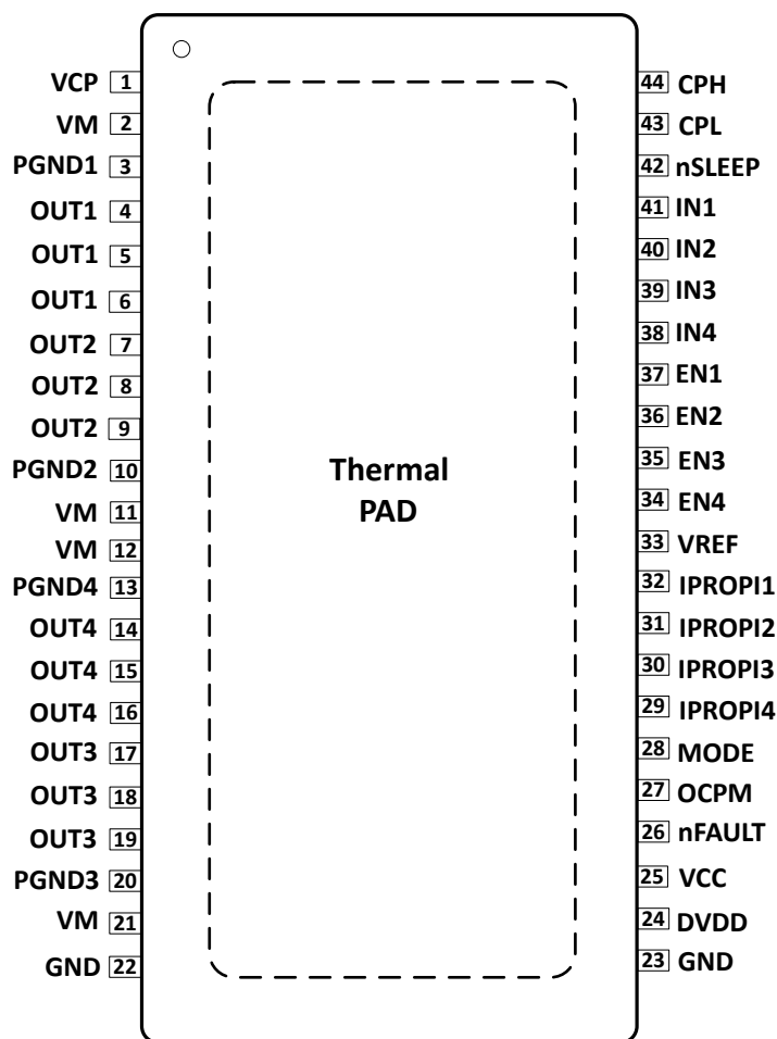
Figure 4-1. Top View
