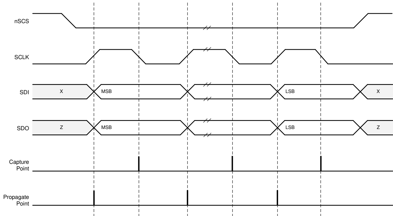
Figure 7-32. SPI Transaction
