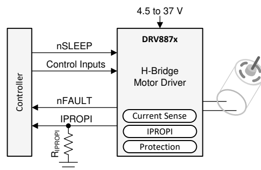
Simplified Schematic
