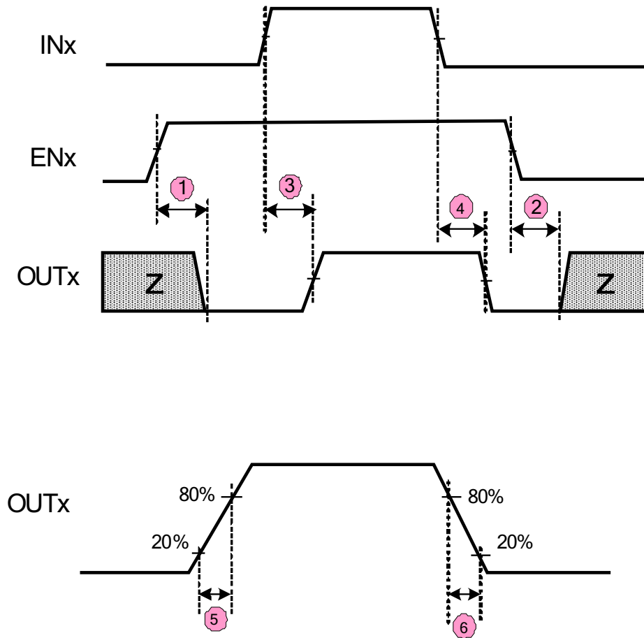
Figure 1. Timing Requirements
