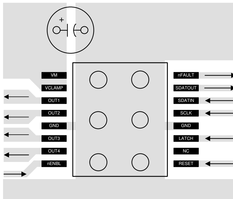
Figure 8-7. Layout Recommendation
