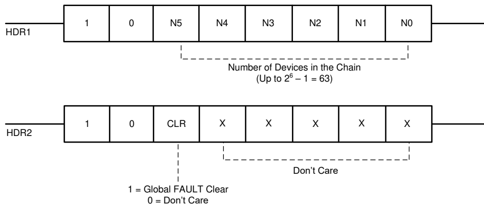
Figure 7-35. Header Bits
