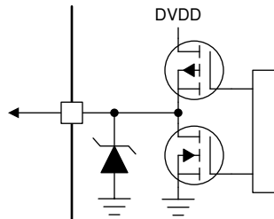
Figure 6-15. Push Pull Output Structure (SDO)
