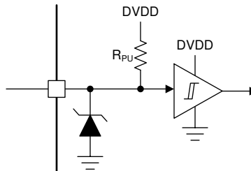
Figure 6-14. Input Pin Structure (nSCS)
