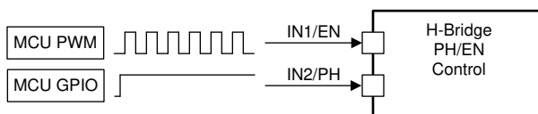
Figure 6-4. H-Bridge PH/EN Control
