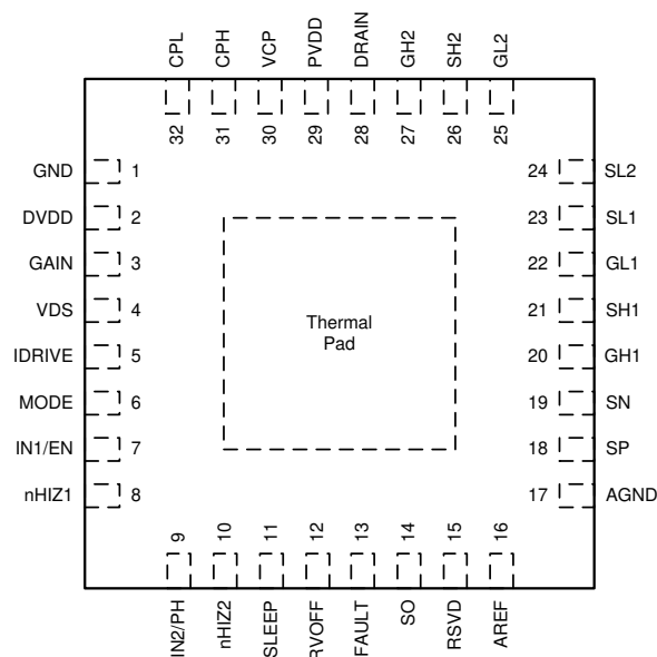
Figure 4-2. DRV8705H-Q1 RHB Package 32-Pin VQFN Top View
