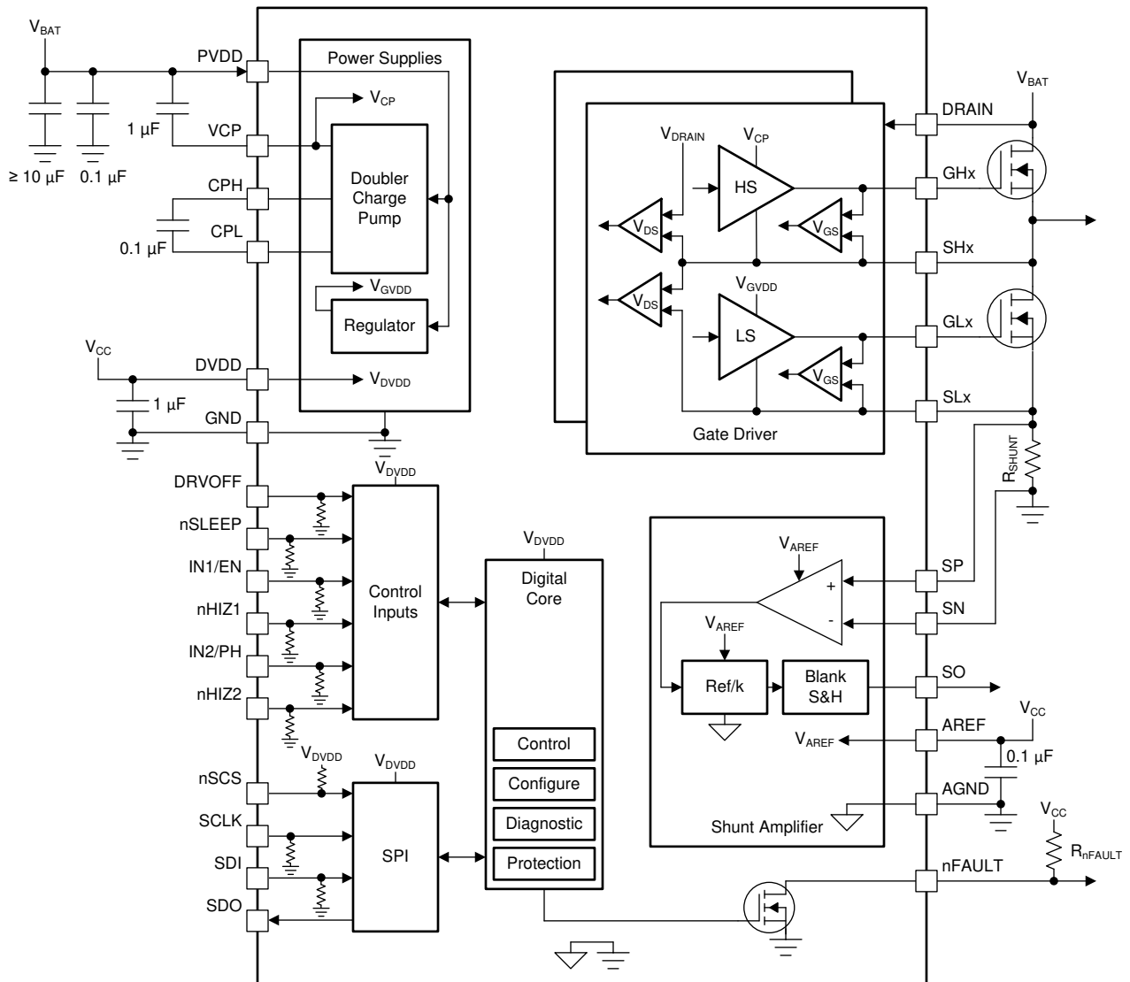
Figure 6-1. DRV8705S-Q1 Functional Block Diagram
