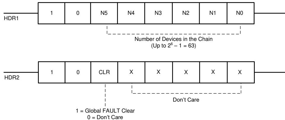
Figure 6-24. Header Bits
