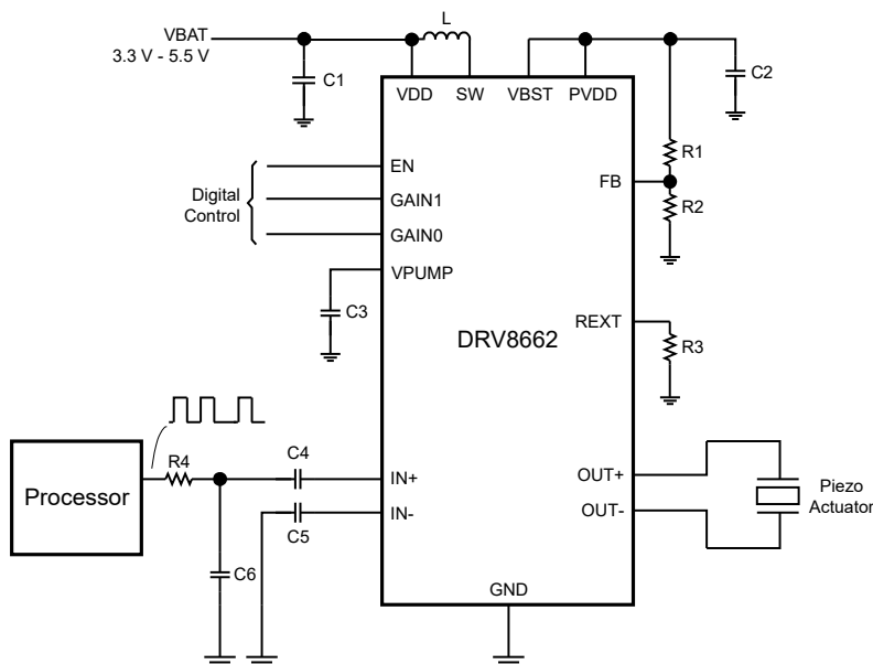
Figure 8-4. DRV8662 System Diagram with Filtered Single-Ended PWM Input
