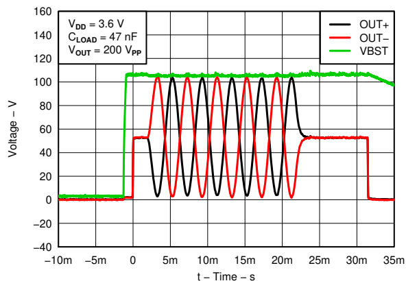
Figure 6-8. Typical Waveform
