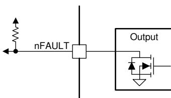
Figure 6-11. nFAULT Pin
