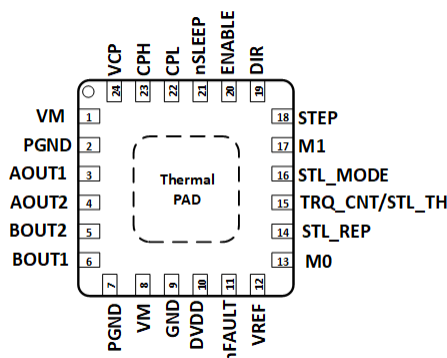
Figure 4-1. RGE Package 24-Pin VQFN with Exposed Thermal PAD Top View
