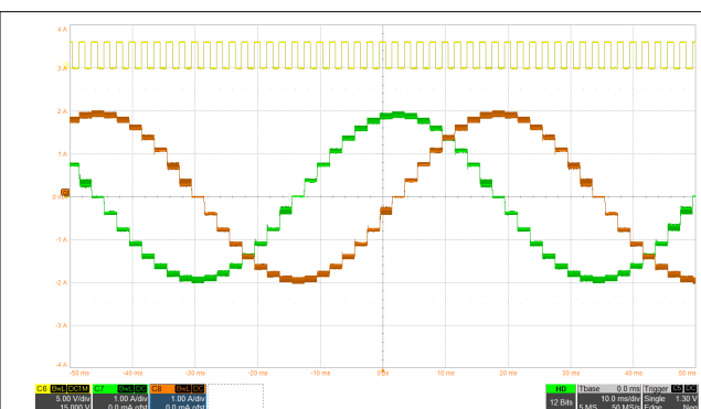
Figure 8-4. 1/8 Microstepping With smart tune Dynamic Decay
