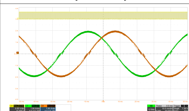
Figure 8-6. 1/32 Microstepping With smart tune Dynamic Decay
