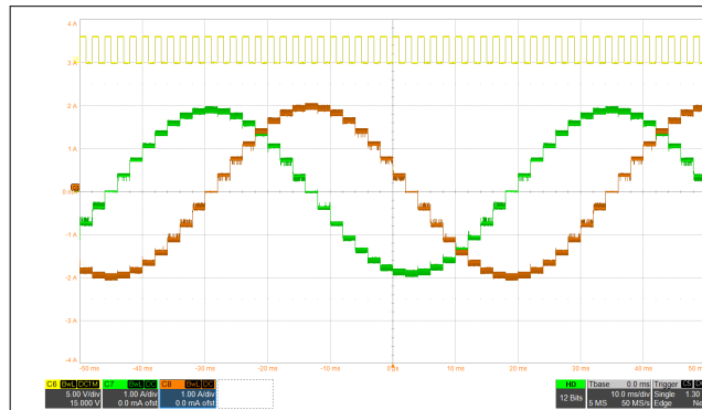
Figure 8-2. 1/8 Microstepping With smart tune Ripple Control Decay
