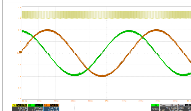
Figure 8-4. 1/32 Microstepping With smart tune Ripple Control Decay
