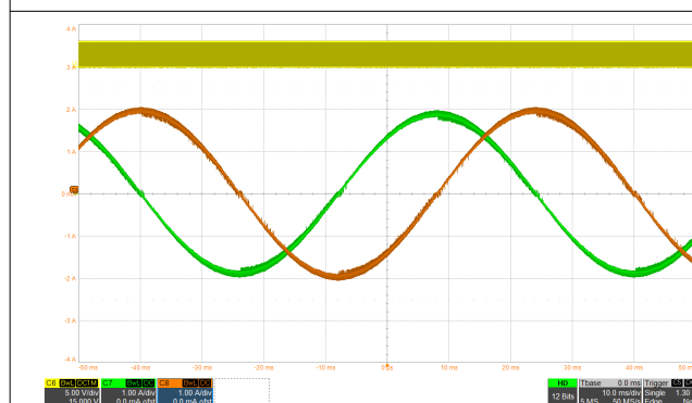
Figure 8-6. 1/256 Microstepping With smart tune Ripple Control Decay
