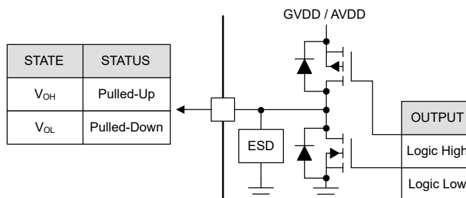
Figure 7-18. Push Pull
