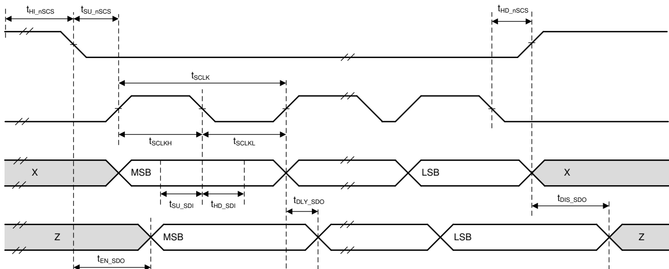
Figure 6-1. SPI Slave Mode Timings
