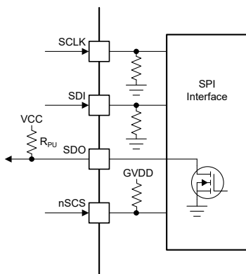
Figure 7-5. DRV8376S SPI
