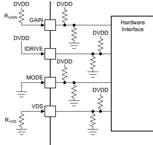
Figure 17. Hardware Interface
