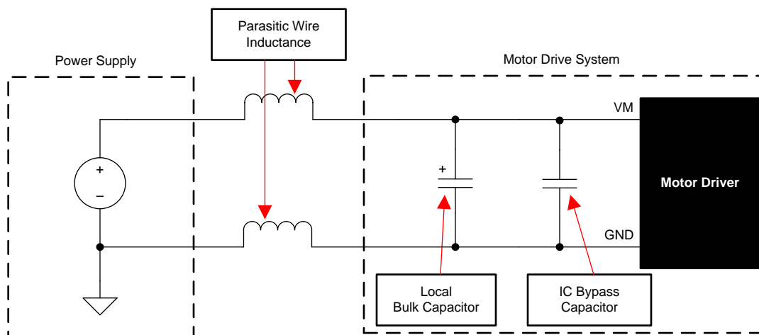
Figure 68. Motor Drive Supply Parasitics Example
