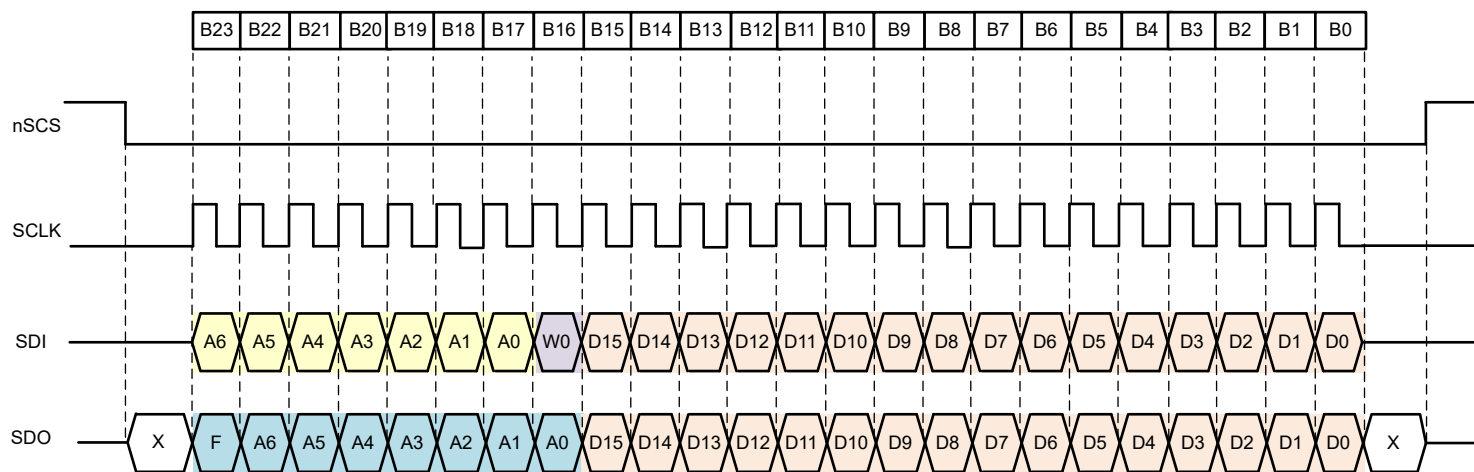
Figure 6-26. SPI Format - 24-bit frame (SPI_CRC_EN = 0b)
