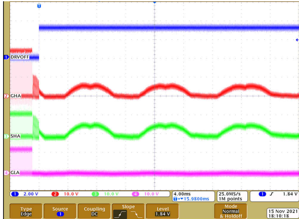
Figure 9-13. DRVOFF operation
