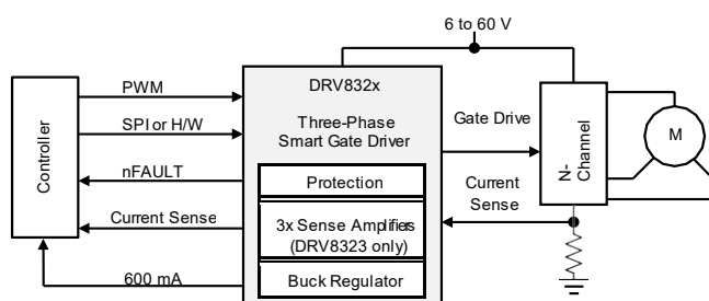
Simplified Schematic
