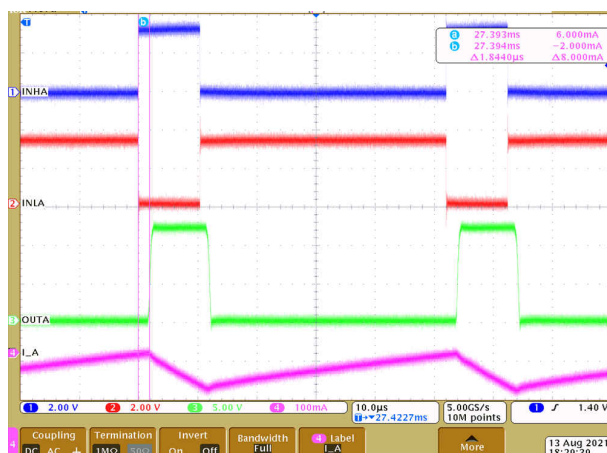
Figure 9-9. Driver delay compensation (1.8 µs)
