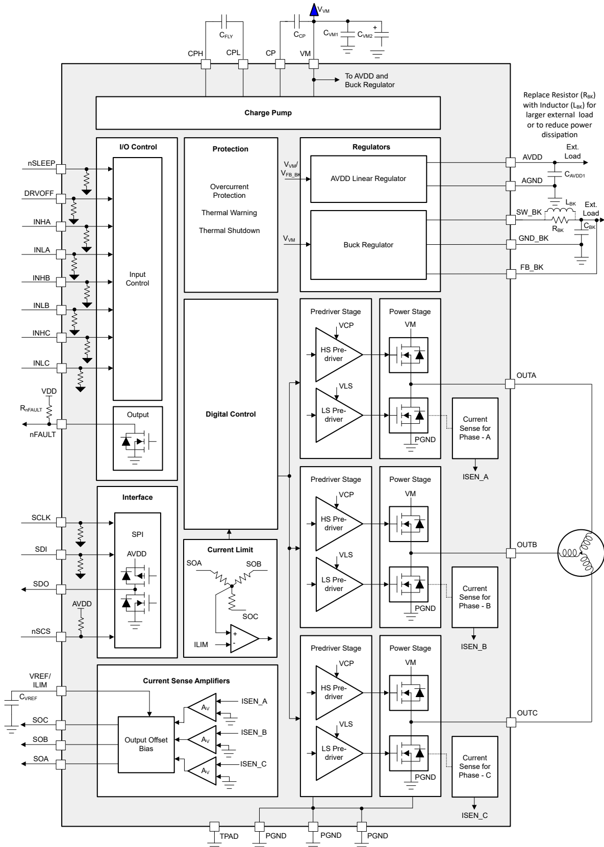
Figure 8-1. DRV8316C-Q1 Block Diagram
