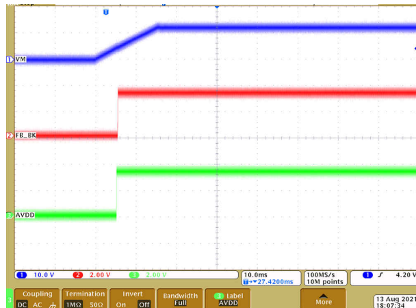
Figure 9-7. Power management
