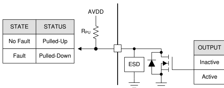
Figure 8-25. Open Drain
