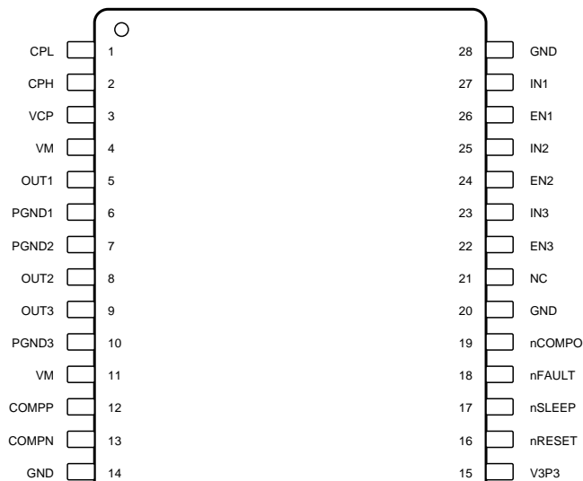
PWP Package 28-Pin HTSSOP With PowerPAD Package Top View
