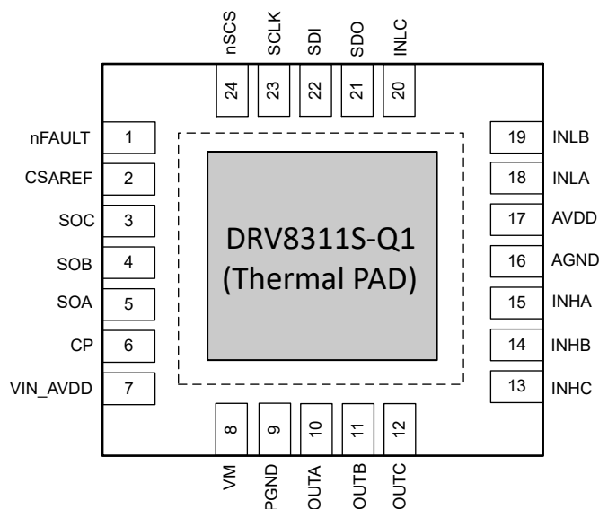
Figure 5-1. DRV8311S-Q1 24-Pin WQFN With Exposed Thermal Pad Top View
