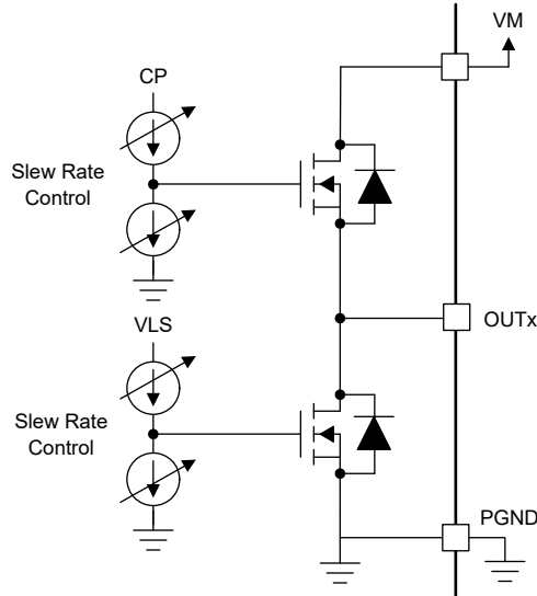
Figure 7-18. Slew Rate Circuit Implementation
