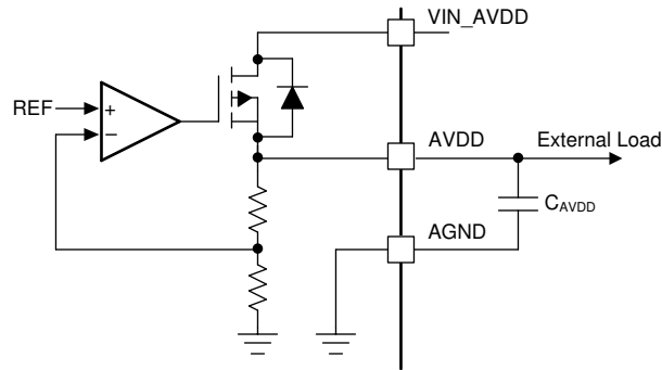
Figure 7-16. AVDD Linear Regulator Block Diagram
