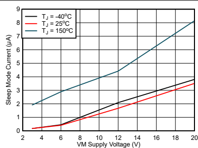
Figure 6-4. Sleep current over supply voltage
