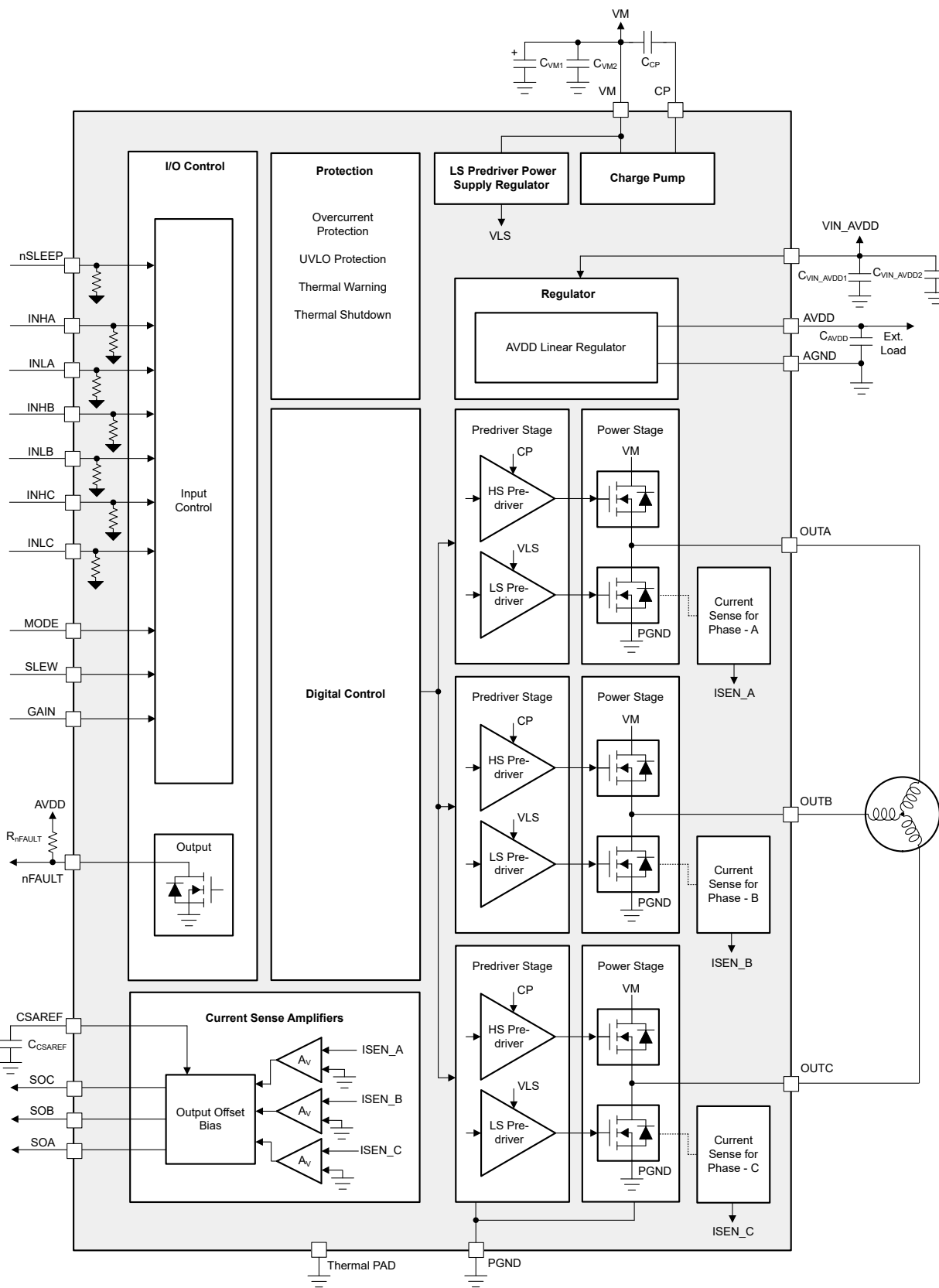
Figure 7-2. DRV8311H-Q1 Block Diagram
