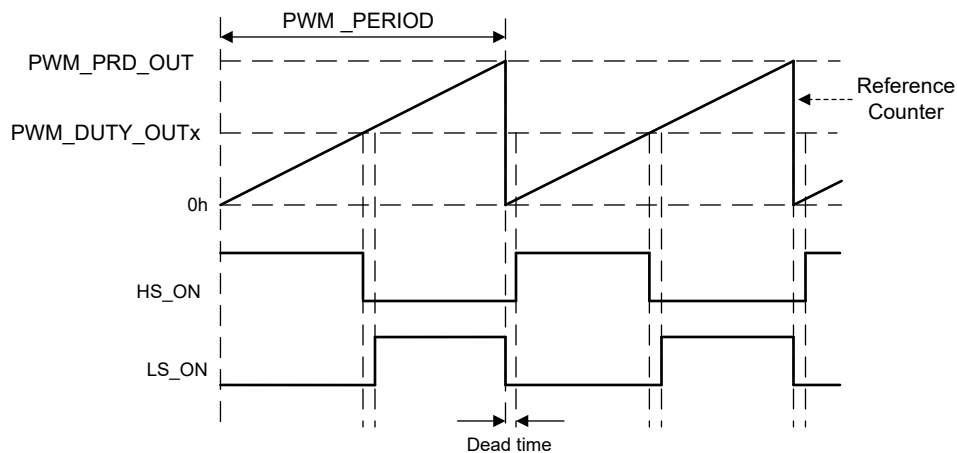
Figure 7-9. PWM Generation - Up Mode
