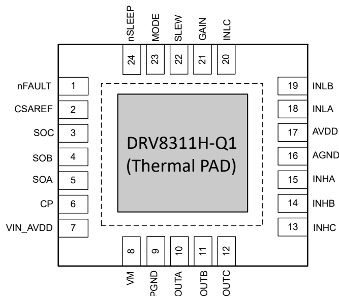
Figure 5-2. DRV8311H-Q1 24-Pin WQFN With Exposed Thermal Pad Top View
