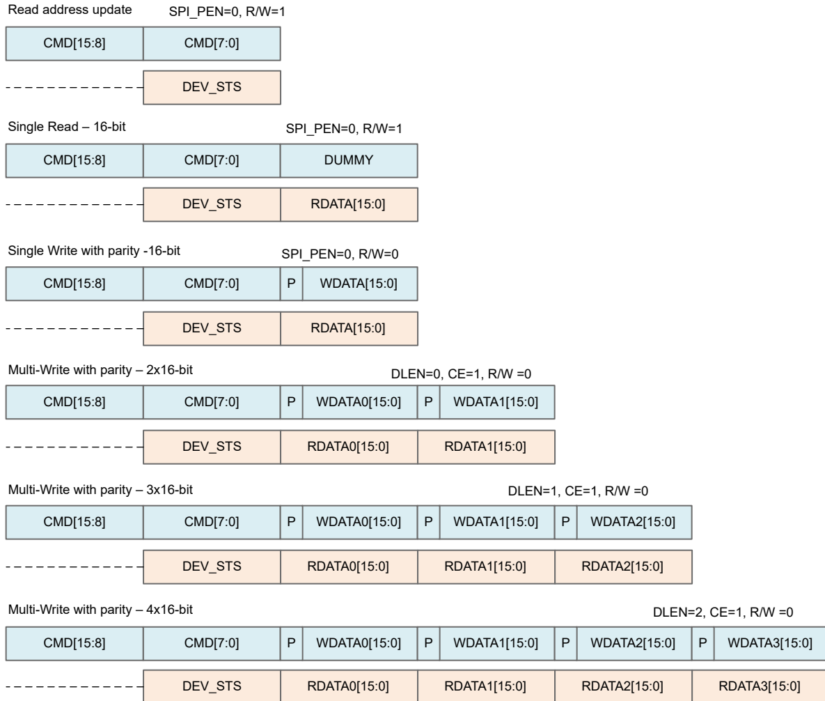
Figure 7-36. tSPI Read/Write with Parity
