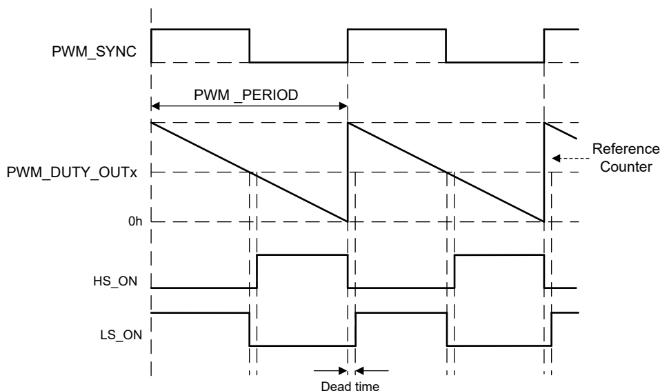
Figure 7-13. PWM Synchronization in Down Mode (PWM_OSC_SYNC = 2h)
