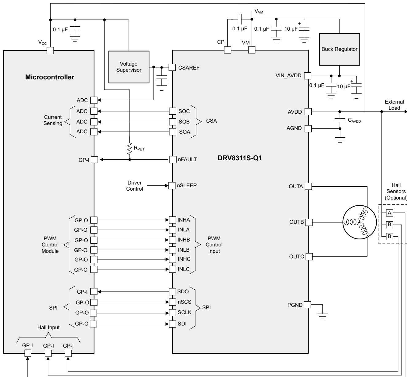
Figure 9-1. Application Schematics (DRV8311S-Q1)
