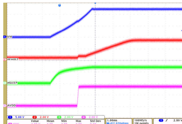
Figure 9-2. Device Power up with VM (VM, nFAULT, nSLEEP, AVDD)
