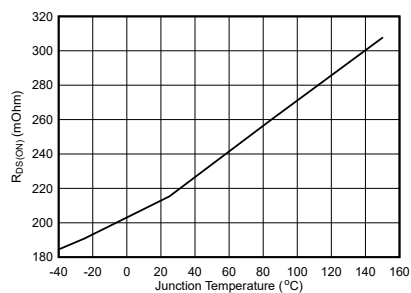
Figure 6-2. R_{DS(ON)} (high and low side combined) for MOSFETs over temperature, V_M \geq 6V
