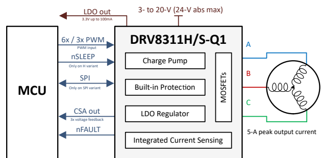
DRV8311H/S-Q1 Simplified Schematic
