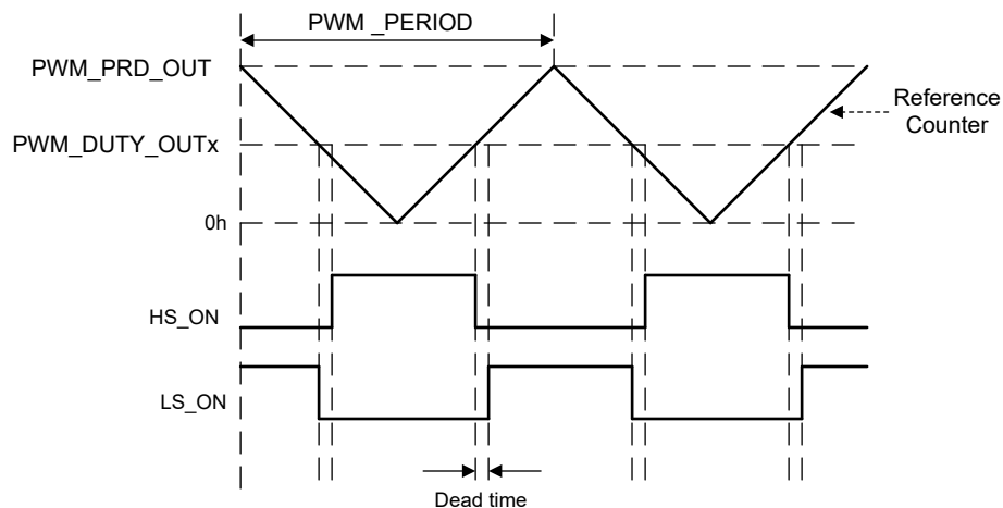
Figure 7-8. PWM Generation - Up/Down Mode
