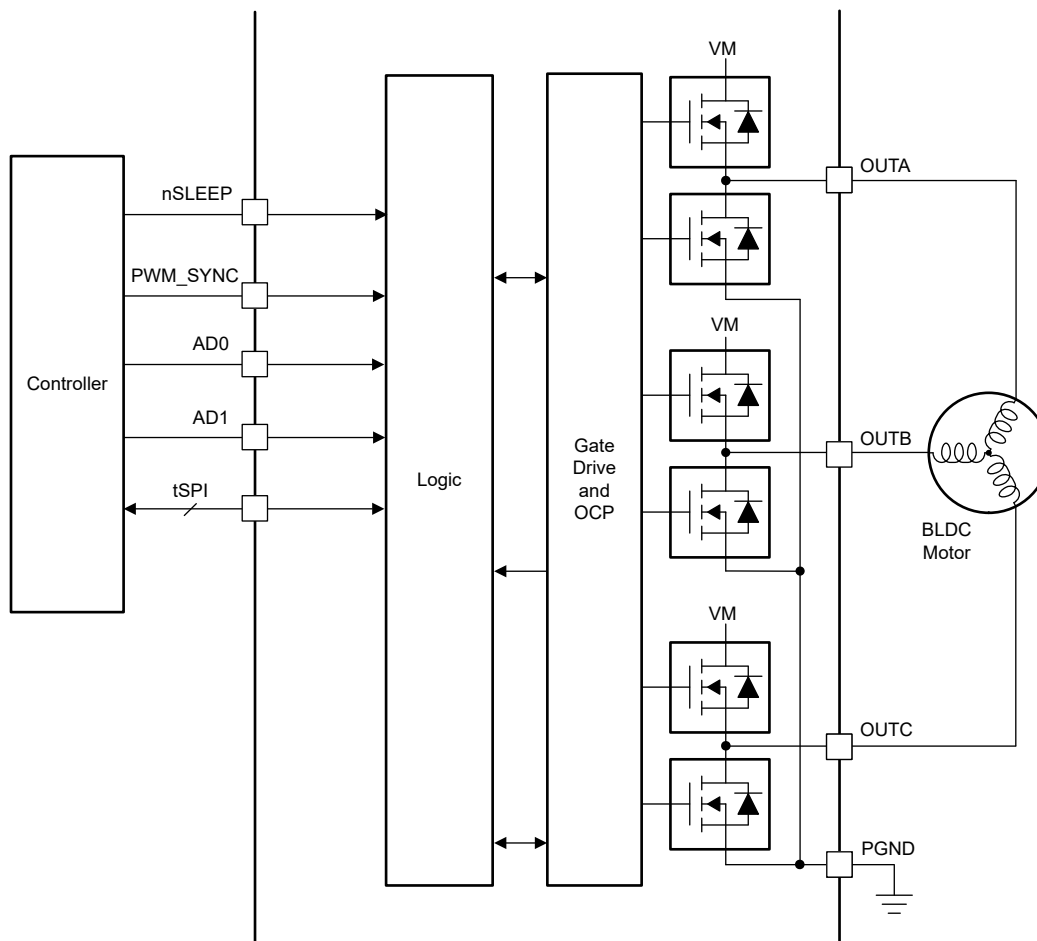
Figure 7-6. PWM Generation Mode - DRV8311P-Q1
