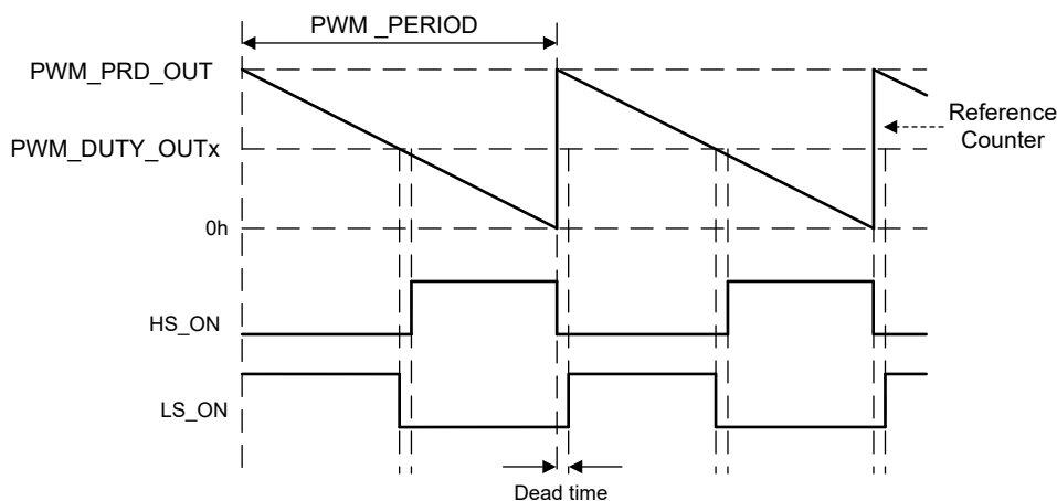
Figure 7-10. PWM Generation - Down Mode
