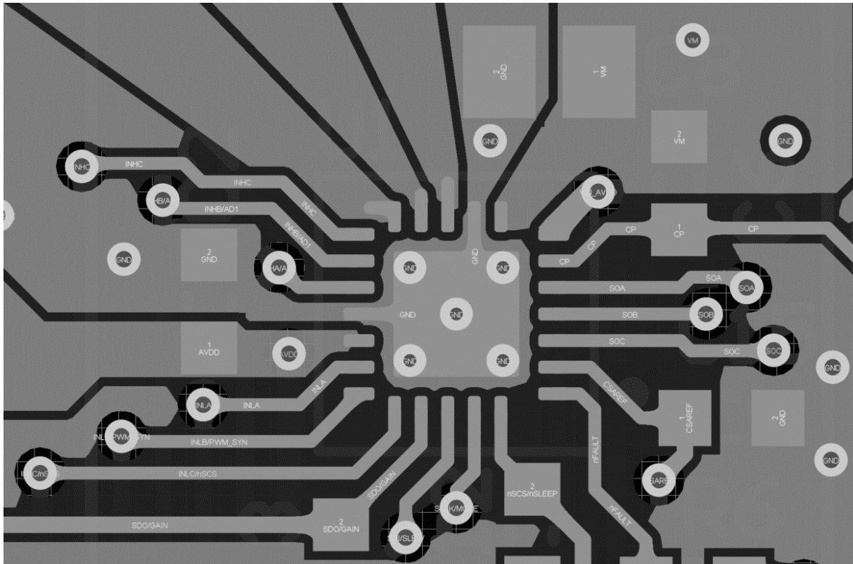
Figure 9-10. Recommended Layout Example for DRV8311-Q1
