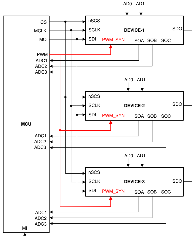
Figure 7-35. tSPI with PWM_SYNC
