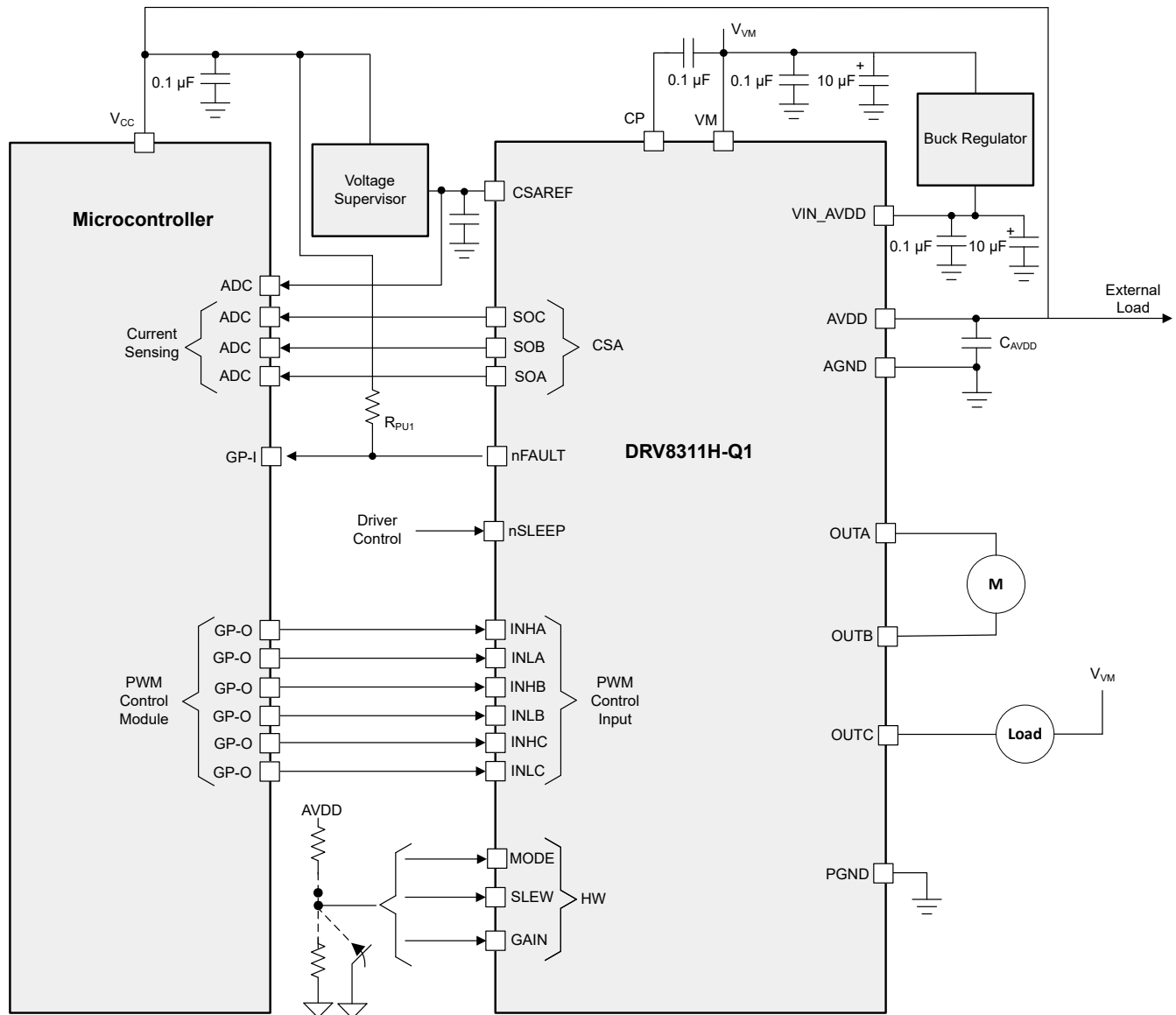
Figure 9-8. Application Schematics (DRV8311H-Q1) - Brushed-DC and Solenoid Load Drive Block Diagram
