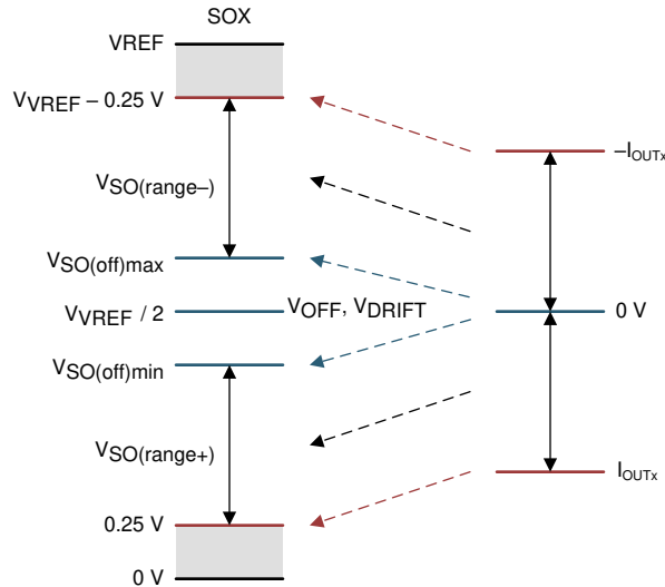
Figure 7-29. Bidirectional Current Sense Output
