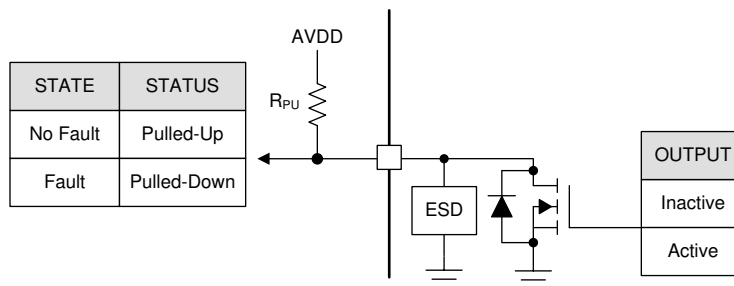
Figure 7-25. Open Drain Output Pin Structure
