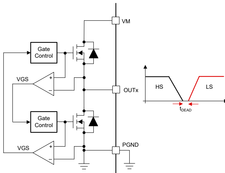
Figure 7-20. Cross Conduction Protection
