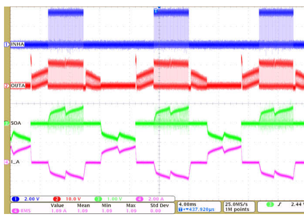
Figure 9-5. Driver PWM Operation with Current Sense Feedback (INHA, OUTA, SOA, I_A)
