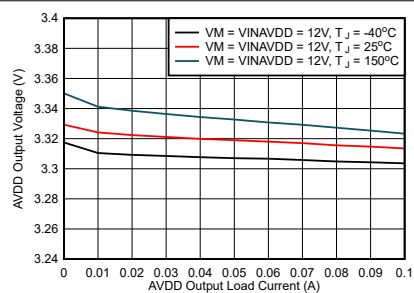
Figure 6-5. AVDD regulator output voltage over load current
