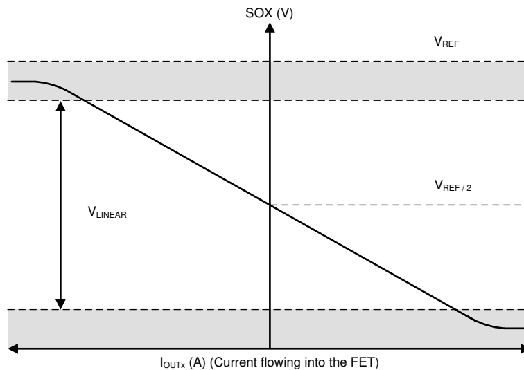
Figure 7-30. Bidirectional Current Sense Regions
