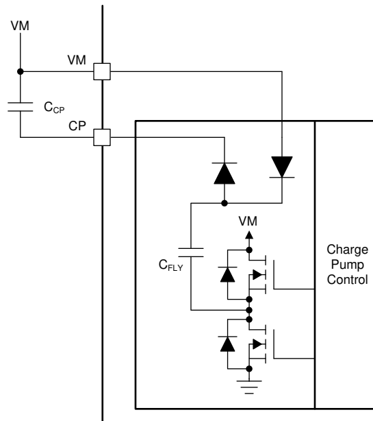
Figure 7-17. The Charge Pump
