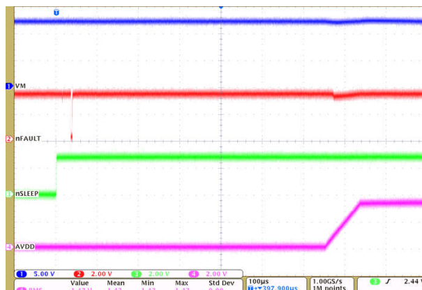
Figure 9-3. Device Power up with nSLEEP (VM, nFAULT, nSLEEP, AVDD)
