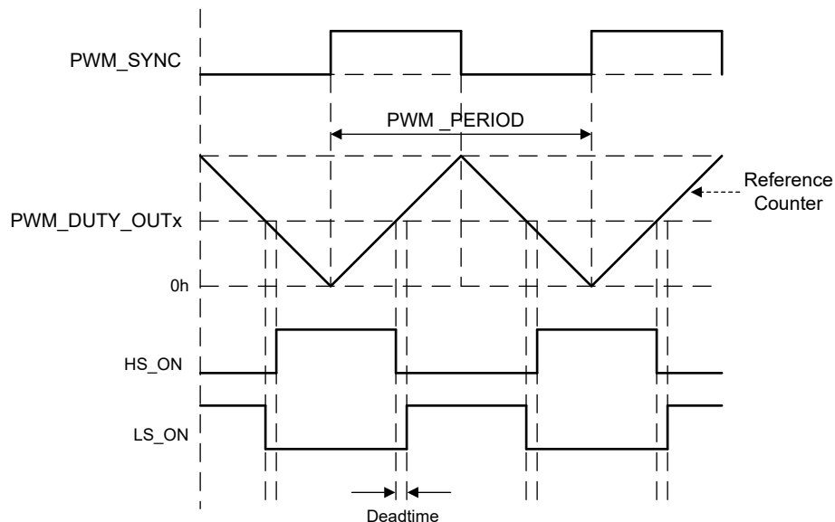
Figure 7-11. PWM Synchronization in Up/down Mode (PWM_OSC_SYNC = 2h)
