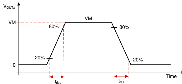
Figure 7-19. Slew Rate Timings
