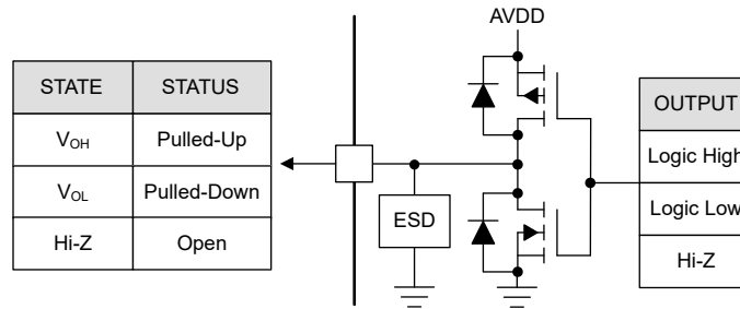
Figure 7-26. Push-Pull Output Pin Structure
