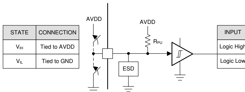
Figure 7-24. nSCS Input Pin Structure
