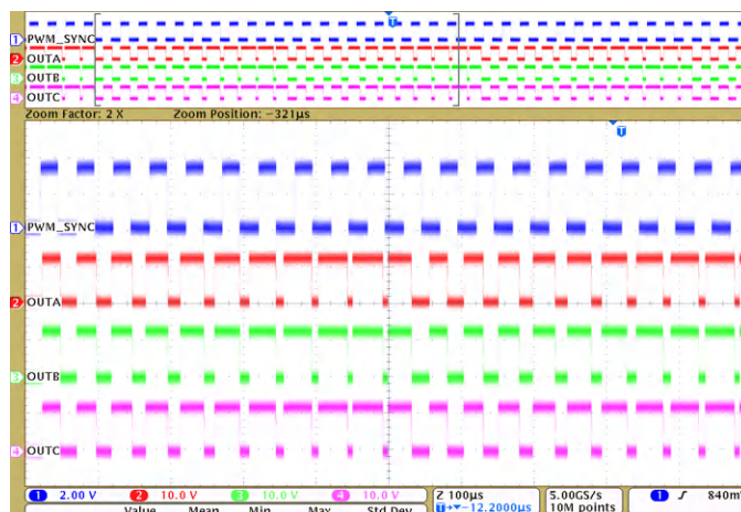
Figure 9-7. PWM Synchronous Duty Cycle Operation with PWM_SYNC = 2b (10% - 90%) (PWM_SYNC, OUTA, OUTB, OUTC)
