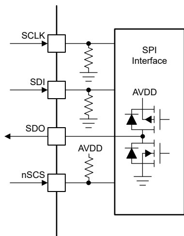
Figure 7-14. DRV8311P/S-Q1 SPI
