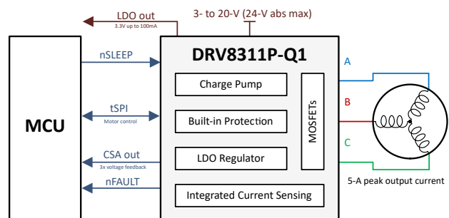
DRV8311P-Q1 Simplified Schematic
