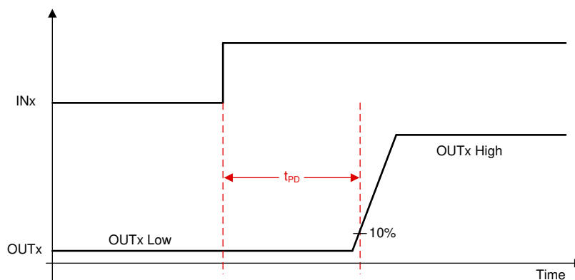
Figure 7-22. Propagation Delay
