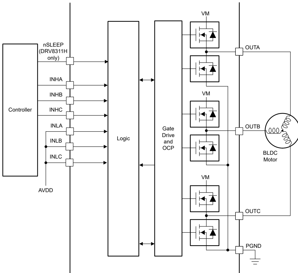
Figure 7-5. 3x PWM Mode
