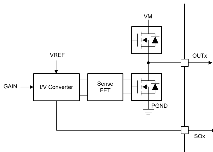
Figure 7-28. Integrated Current Sense Amplifier
