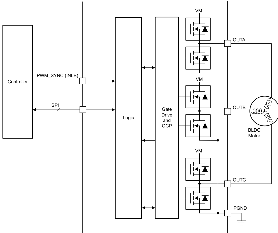
Figure 7-7. PWM Generation Mode - DRV8311S-Q1
