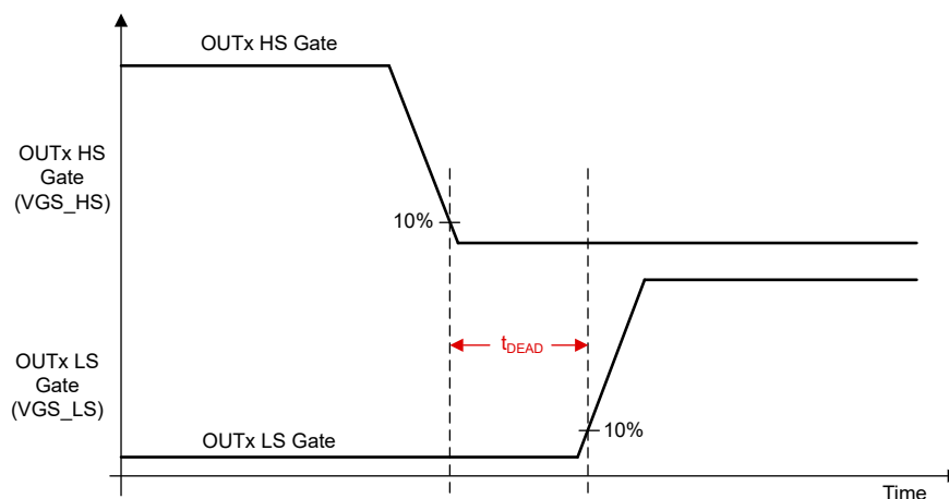
Figure 7-21. Dead Time
