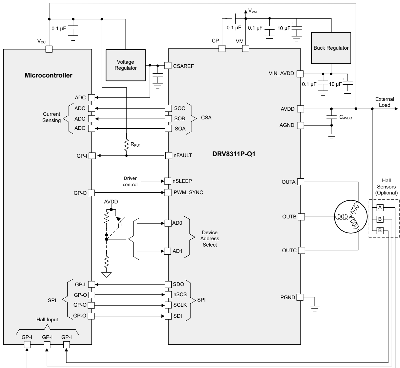
Figure 9-6. Application Schematics (DRV8311P-Q1) - Three Phase Brushless-DC tSPI Motor Control
