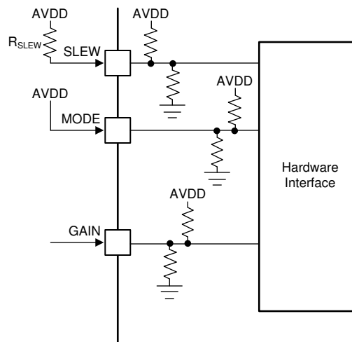
Figure 7-15. DRV8311H-Q1 Hardware Interface
