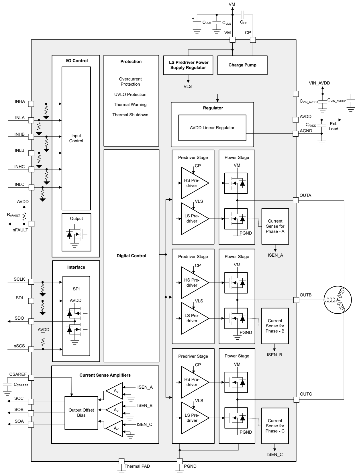
Figure 7-1. DRV8311S-Q1 Block Diagram
