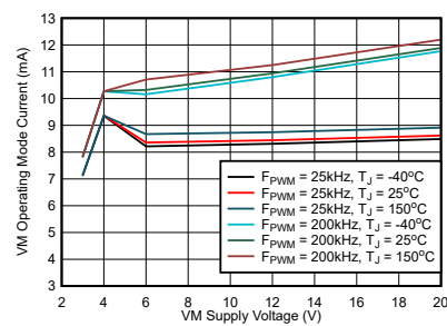
Figure 6-3. Operating mode current over supply voltage
