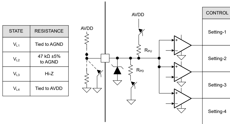
Figure 7-27. Four Level Input Pin Structure
