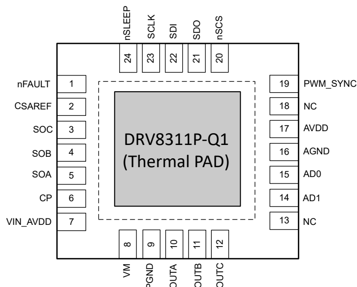
Figure 5-3. DRV8311P-Q1 24-Pin WQFN With Exposed Thermal Pad Top View
