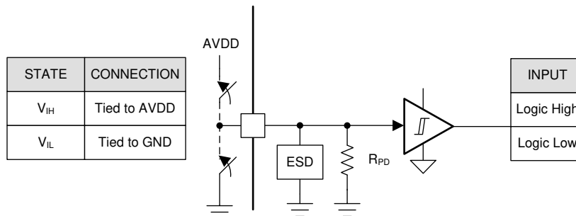
Figure 7-23. Logic-Level Input Pin Structure
