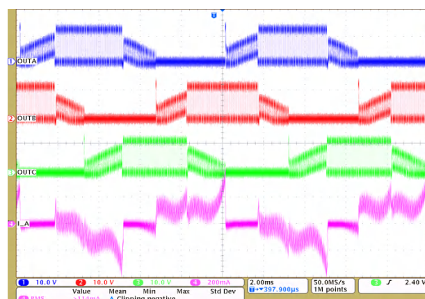
Figure 9-4. Driver PWM Operation (OUTA, OUTB, OUTC, I_A)
