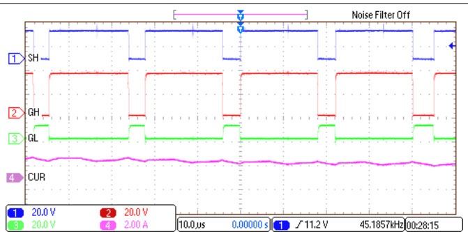
Figure 8. Motor Spinning 4000 RPM
