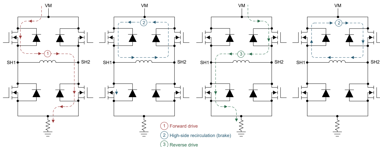
Figure 6-3. Current Paths
