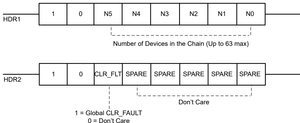
Figure 8-14. Header bytes
