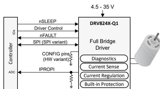
Simplified Schematic
