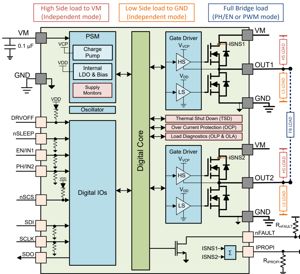
Figure 8-2. Functional Block Diagram - SPI (S) Variant
