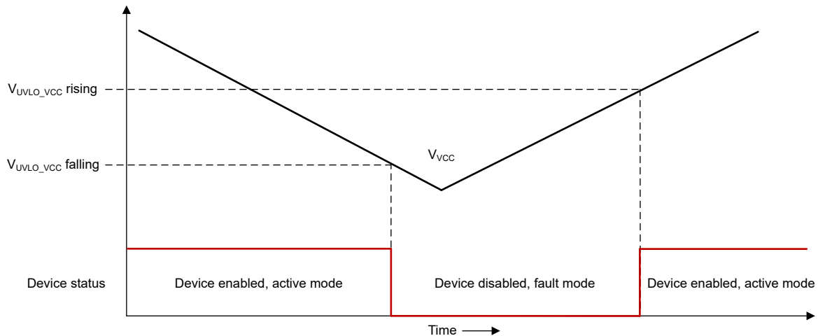
Figure 7-14. UVLO Operation
