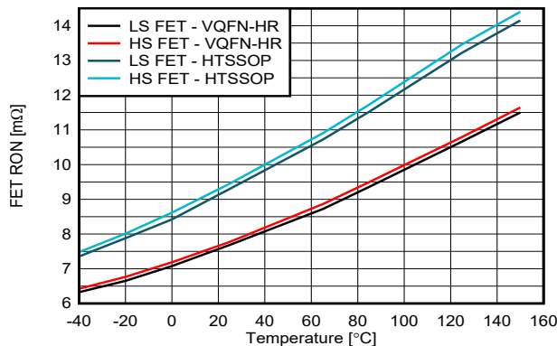
Figure 6-11. R_{HS\_ON} & R_{LS\_ON} vs Temperature at V_{VM} = 13.5\text{ V}
