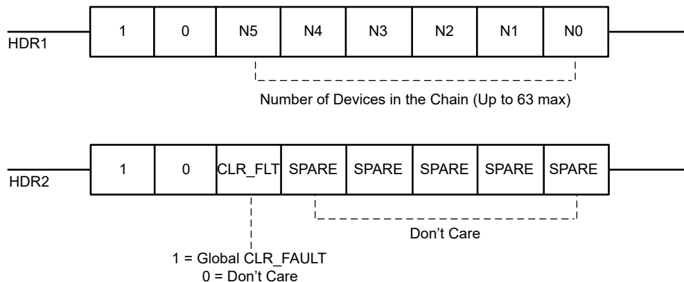
Figure 7-11. Header bytes
