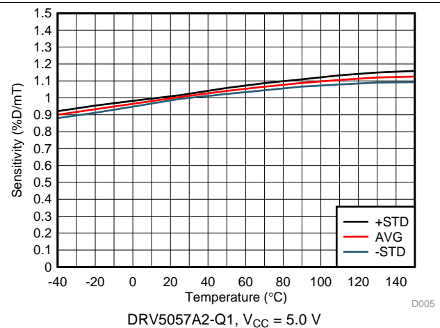
Figure 6. Sensitivity vs Temperature
