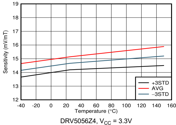
Figure 5-23. Sensitivity vs Temperature
