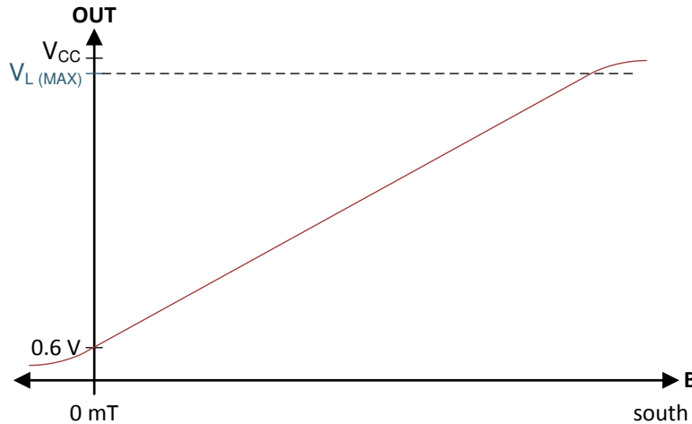
Figure 29. Magnetic Response
