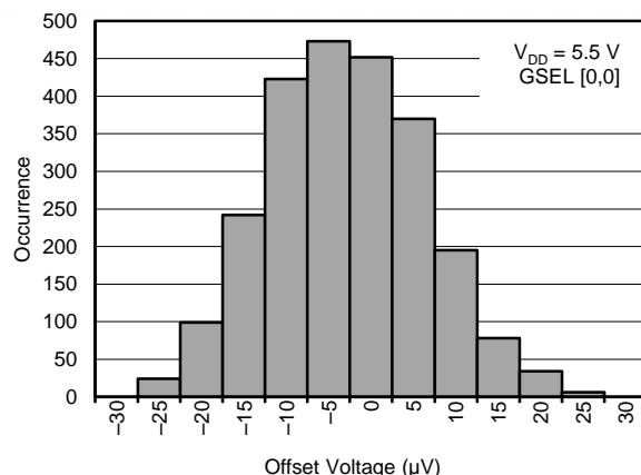
Figure 8. FRONT-END OFFSET VOLTAGE HISTOGRAM
