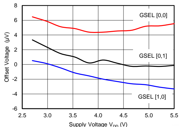
Figure 10. FRONT-END OFFSET VOLTAGE vs POWER SUPPLY
