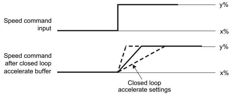
Figure 25. Closed-Loop Accelerate
