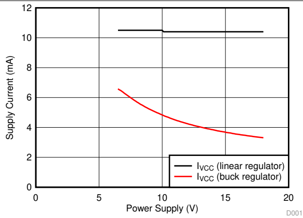
Figure 1. Supply Current vs Power Supply
