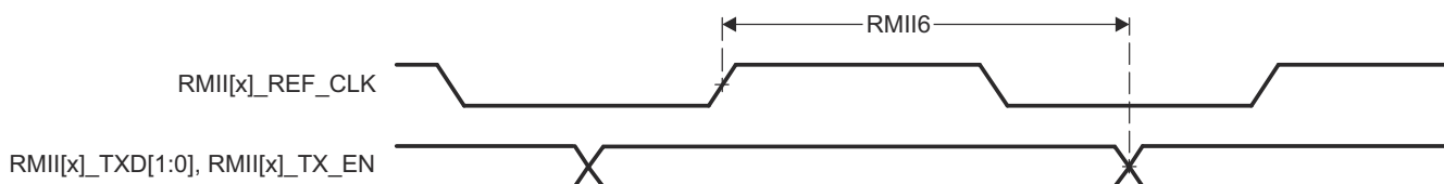
Figure 6-50. RMII[x]_TXD[1:0], and RMII[x]_TX_EN Switching Characteristics – RMII Mode
