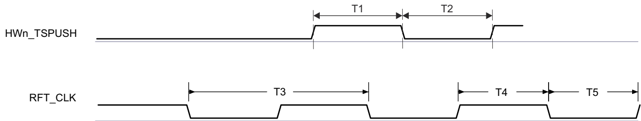
Figure 6-108. CPTS Timing Requirements
