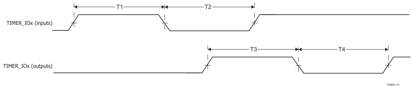
Figure 6-119. Timer Timing
