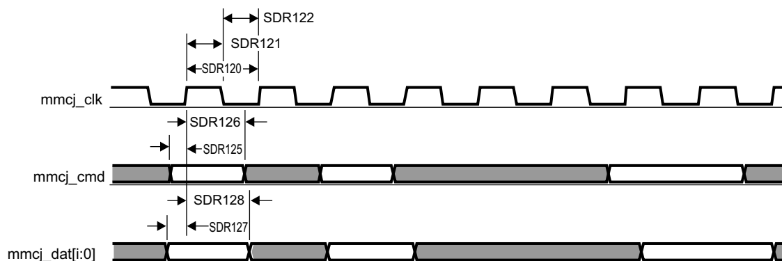
Figure 5-103. MMC/SD/SDIOj in - SDR12 - Receiver Mode
