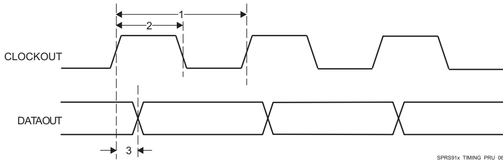
Figure 5-114. PRU-ICSS PRU Shift Out Timing
