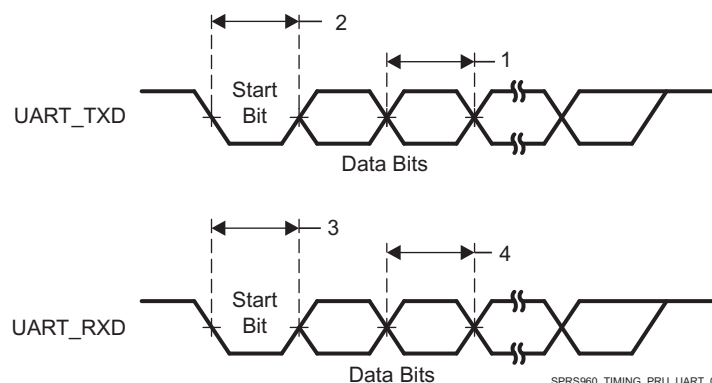
Figure 5-129. PRU-ICSS UART Timing
