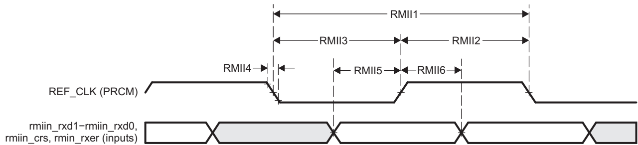
Figure 5-73. GMAC Receive Interface Timing RMII IN operation
