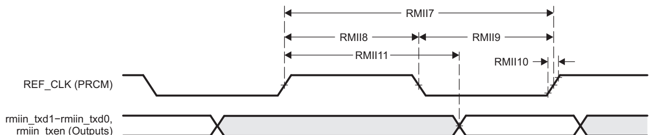
Figure 5-74. GMAC Transmit Interface Timing RMII IN Operation
