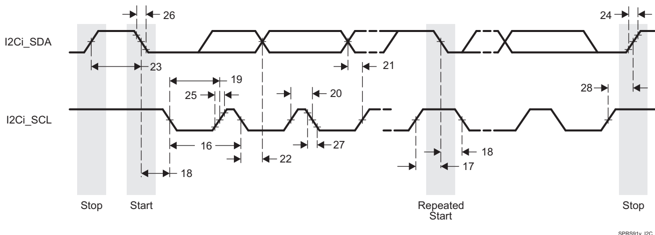
Figure 5-39. I2C Transmit Timing
