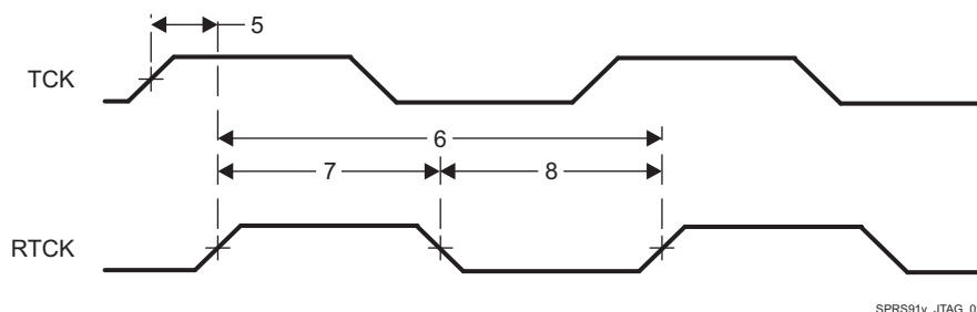
Figure 5-64. JTAG With RTCK Timing
