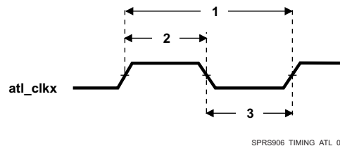
Figure 7-93. ATL_CLKOUTx Timing
