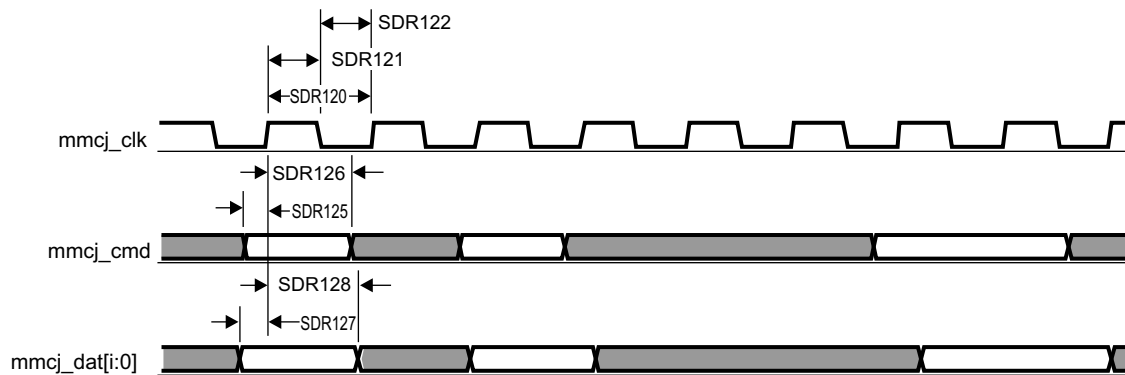
Figure 7-87. MMC/SD/SDIOj in - SDR12 - Receiver Mode
