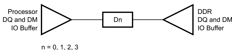
Figure 8-62. DQ/DM Topology
