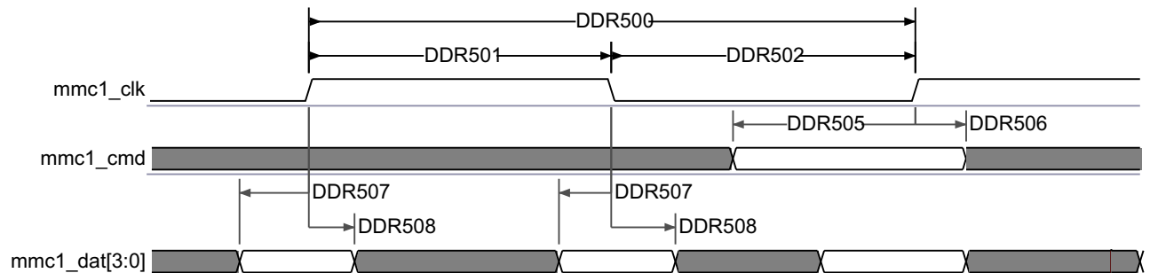
Figure 7-74. SDMMC - High Speed SD - DDR - Data/Command Receive
