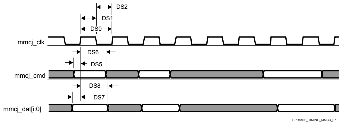
Figure 7-83. MMC/SD/SDIOj in - Default Speed - Receiver Mode
