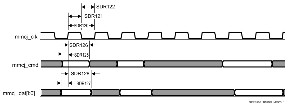
Figure 7-87. MMC/SD/SDIOj in - SDR12 - Receiver Mode
