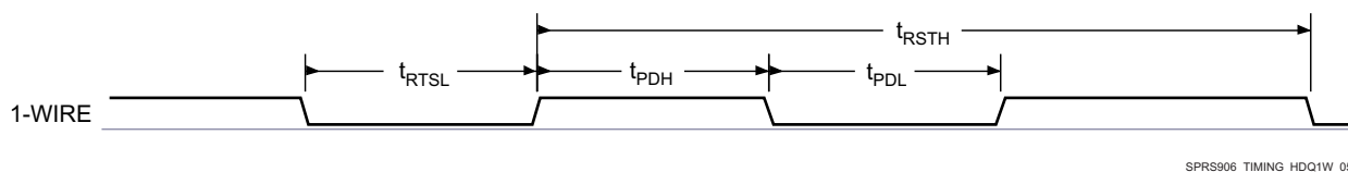
Figure 7-29. 1-Wire-Break (Reset)
