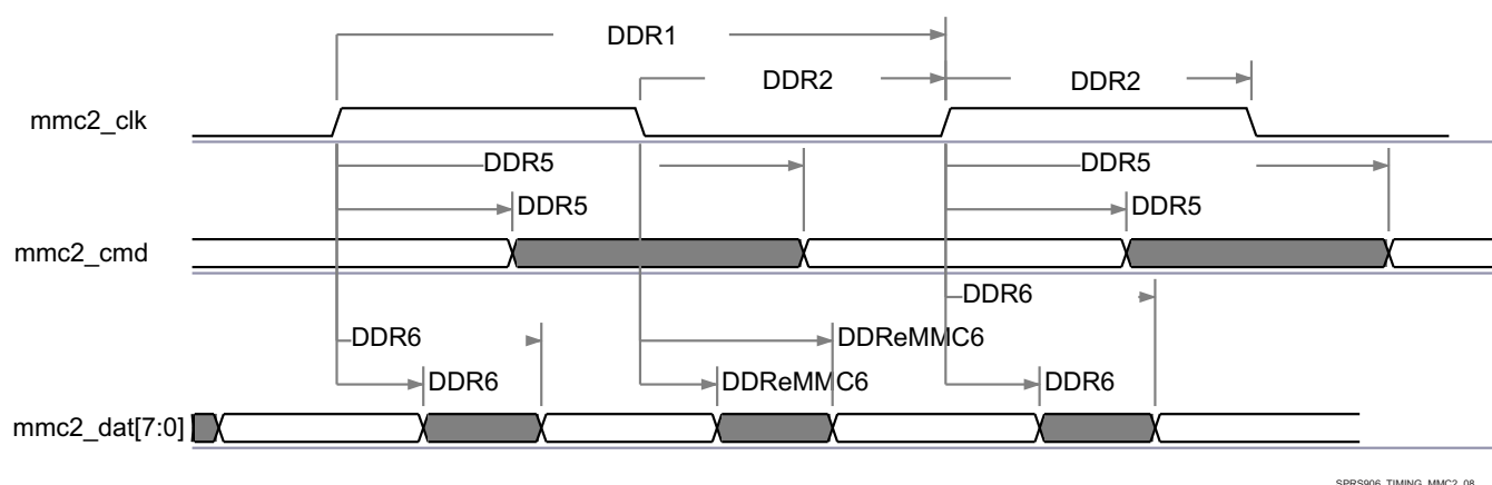
Figure 7-82. MMC/SD/SDIO in - High Speed DDR JC64 - Transmitter Mode
