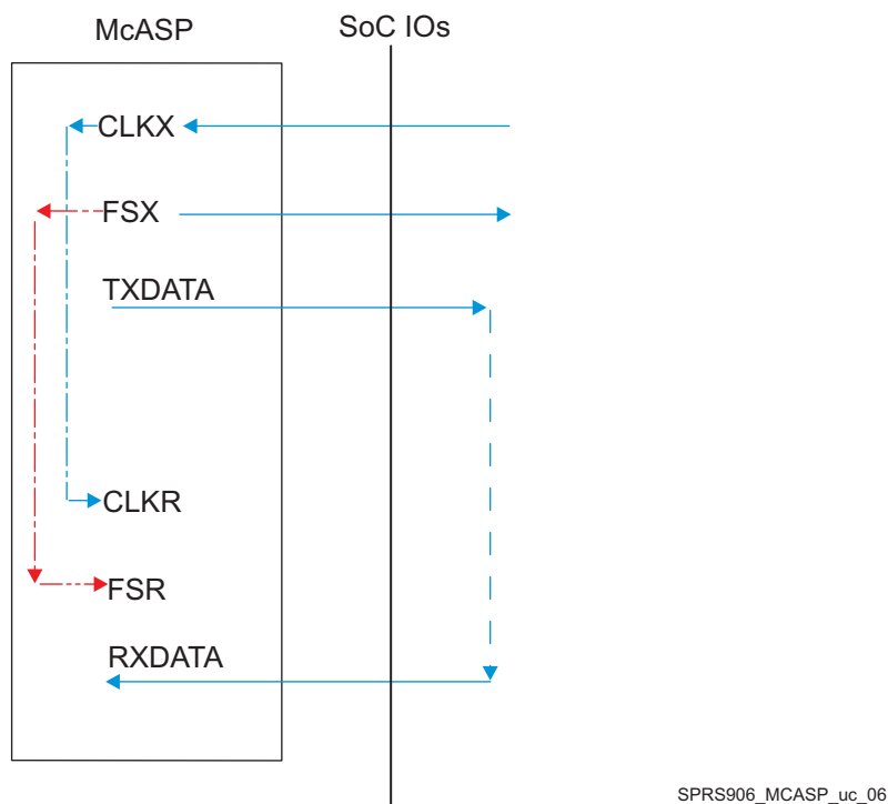
Figure 7-48. McASP1-8 CI-FO- - SYNC Mode
