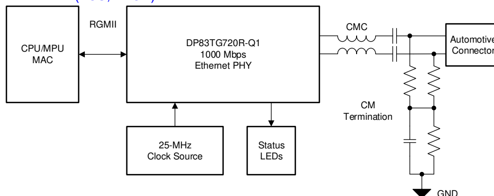
Simplified Schematic
