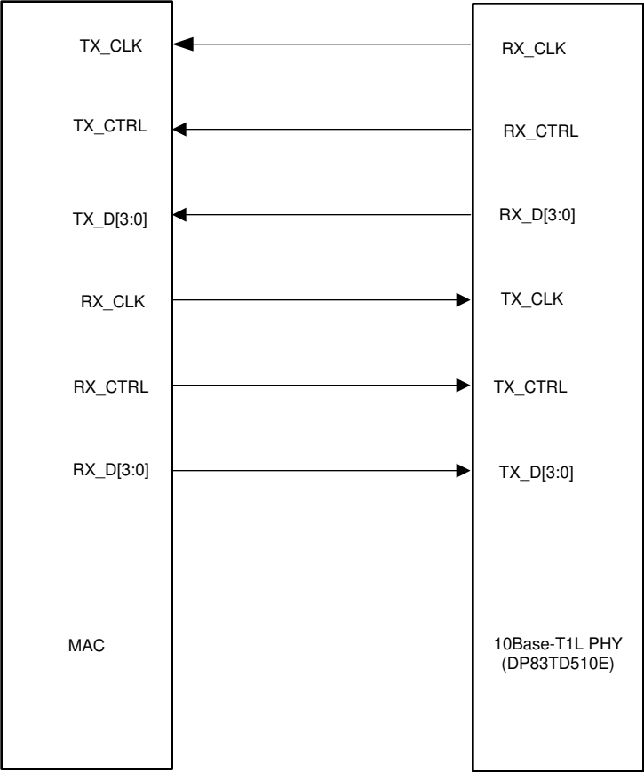
Figure 6-7. RGMII Signalling
