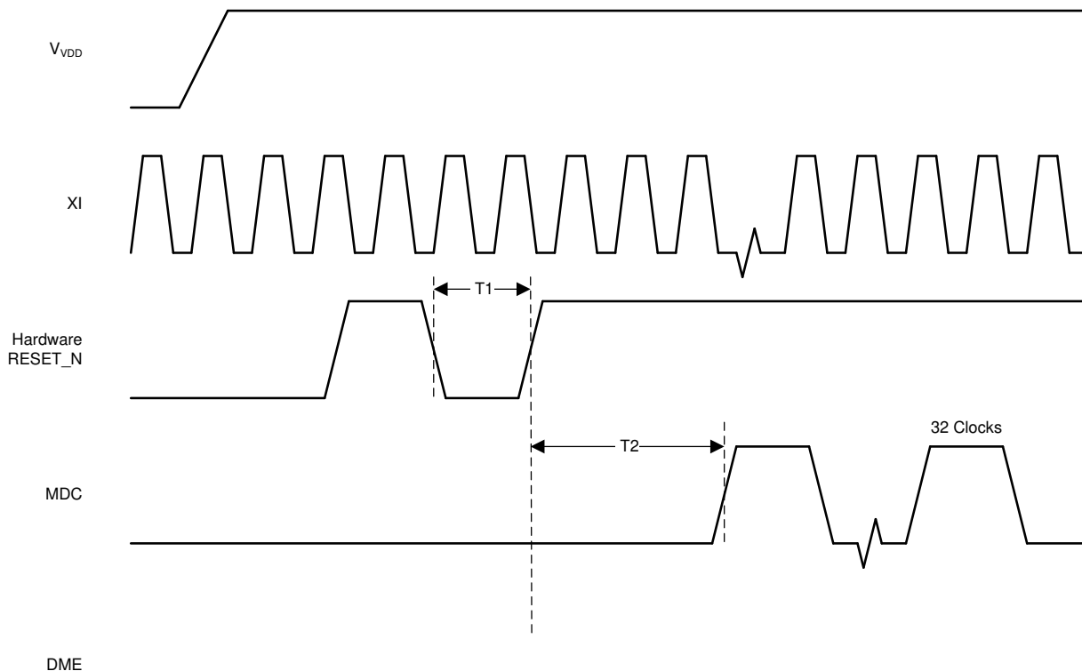
Figure 5-2. Reset Timing
