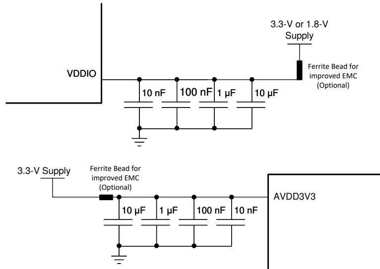
Figure 7-4. DP83825I Power Supply Decoupling Recommendation
