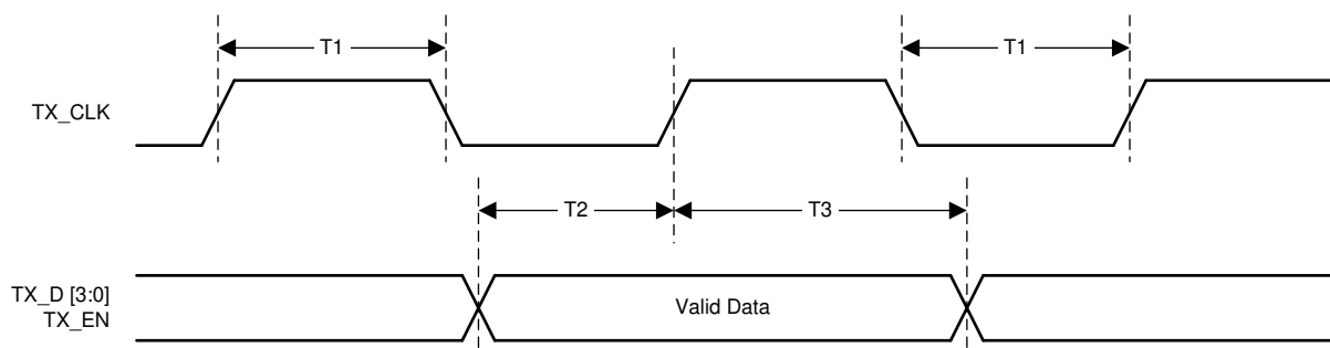
Figure 7-7. 10-Mbps Transmit Timing
