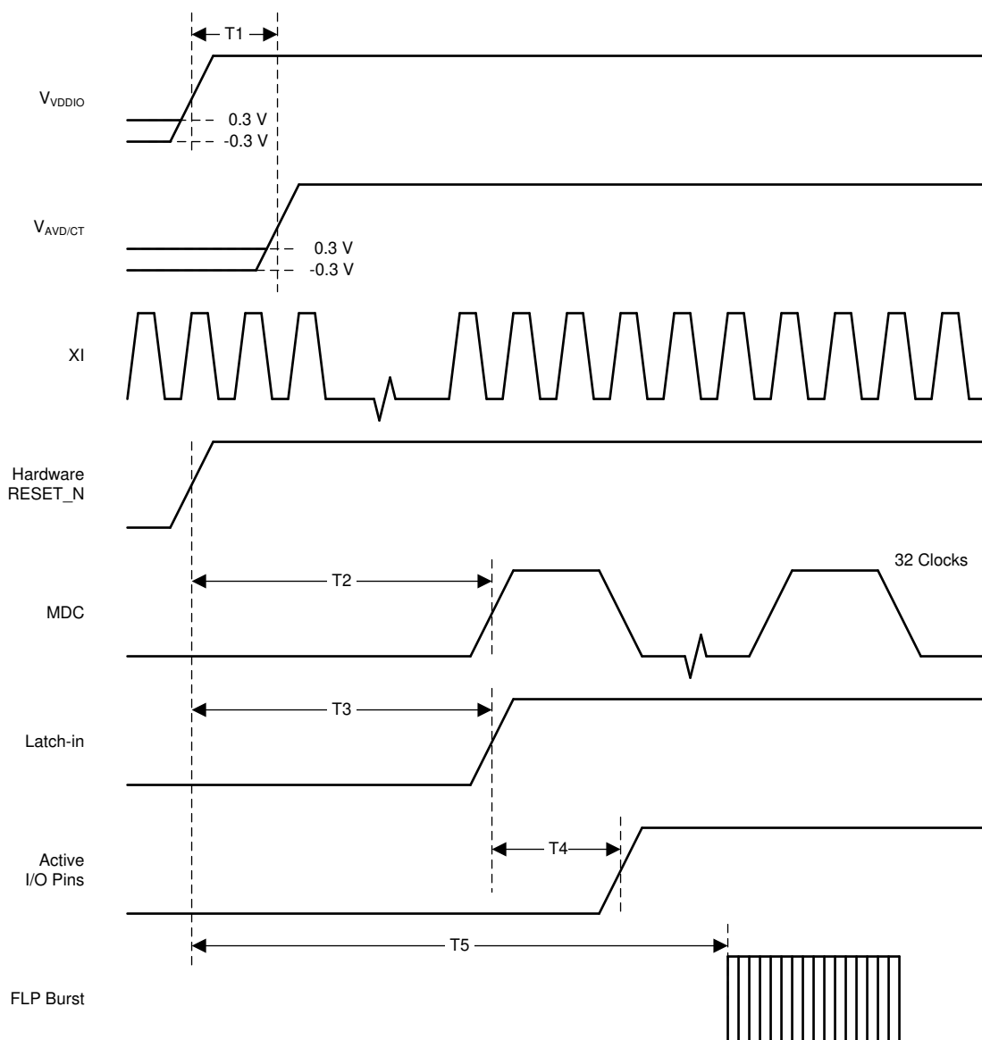
Figure 7-1. Power-Up Timing
