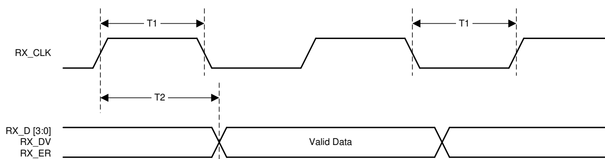
Figure 7-8. 10-Mbps Receive Timing
