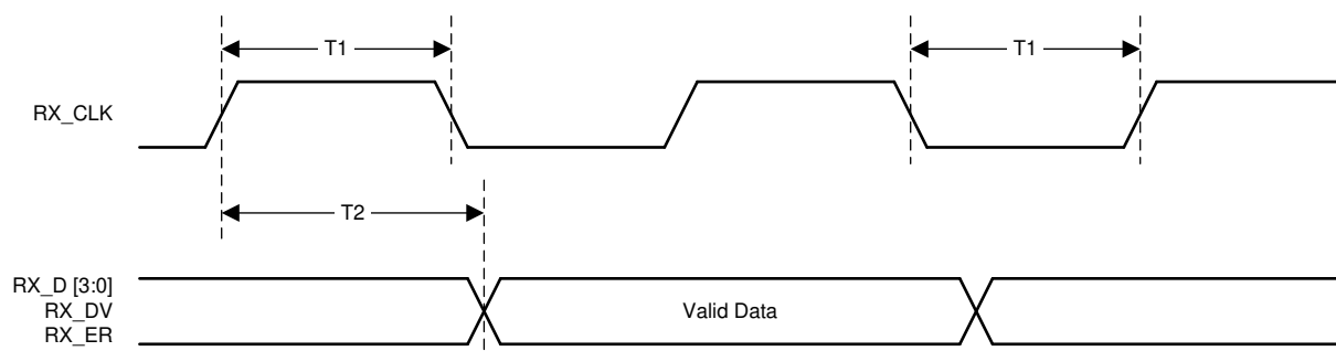
Figure 7-6. 100-Mbps Receive Timing
