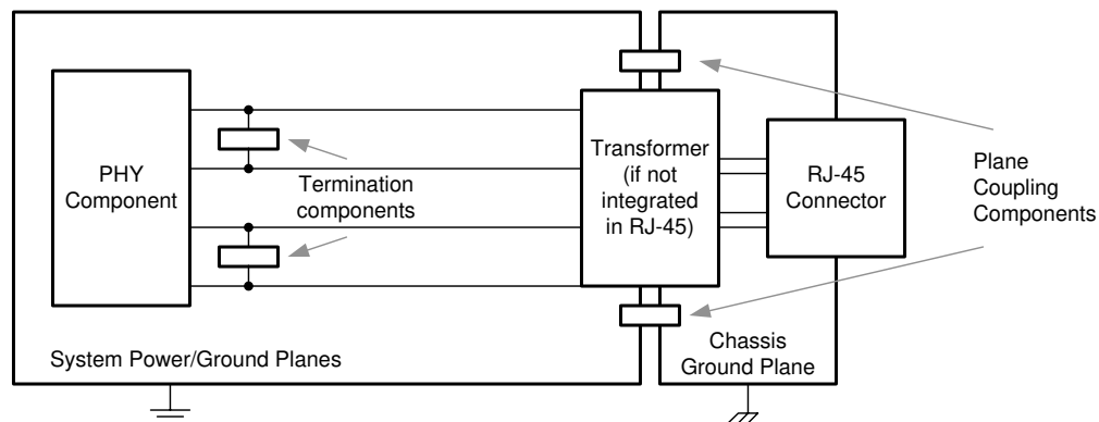
Figure 11-4. Layout Example
