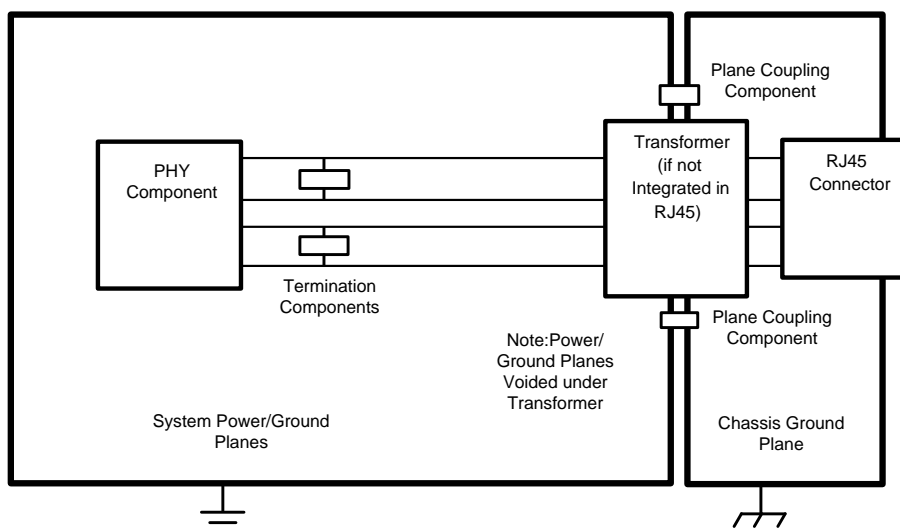
Figure 8-5. Layout Example
