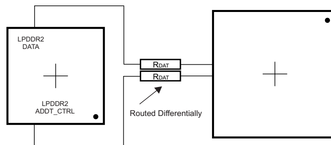
Figure 7-28. DQ[x] Topology
