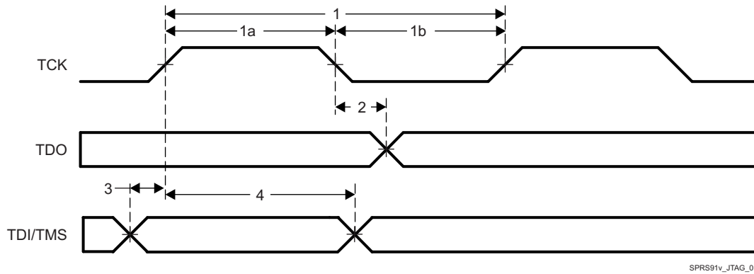
Figure 5-62. JTAG Timing
